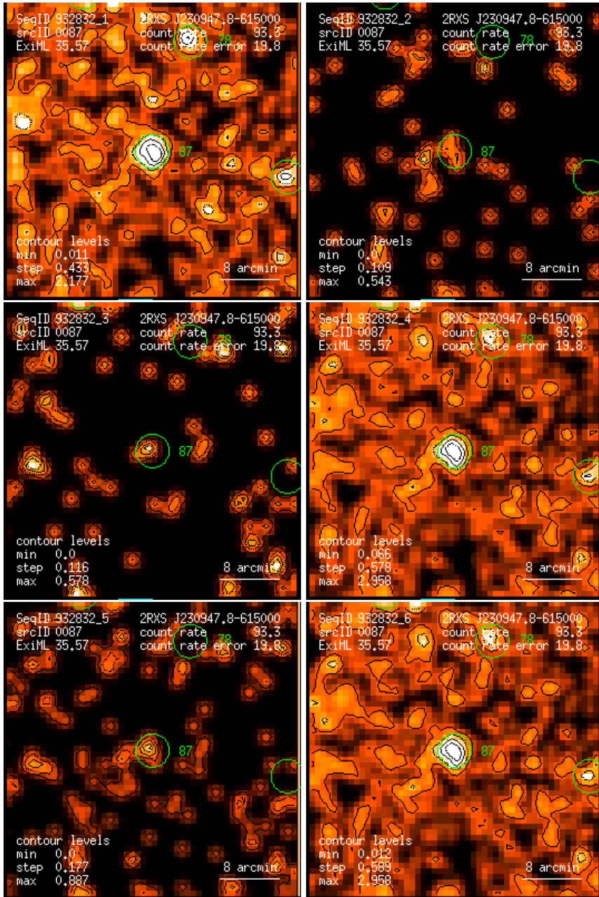
Figure 87: RASS 932832: detection 0087: band rate images, Gaussian filter: (1) PSPC channels 11 – 41, (2) 52 – 90, (3) 91 – 201, (4) 11 – 235, (5) 52 – 201, (6) 11 – 201. Broad band rates in counts/ks. Band rate contour levels in counts/ks/arcmin 2 .
