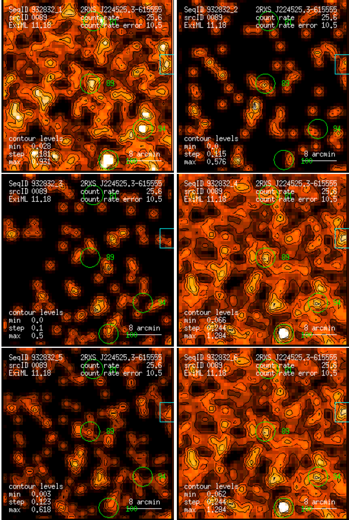
Figure 89: RASS 932832: detection 0089: band rate images, Gaussian filter: (1) PSPC channels 11 – 41, (2) 52 – 90, (3) 91 – 201, (4) 11 – 235, (5) 52 – 201, (6) 11 – 201. Broad band rates in counts/ks. Band rate contour levels in counts/ks/arcmin 2 .
