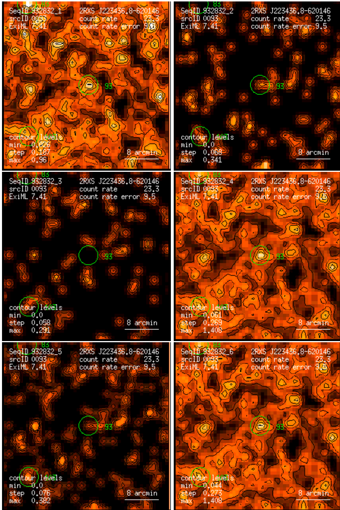
Figure 93: RASS 932832: detection 0093: band rate images, Gaussian filter: (1) PSPC channels 11 – 41, (2) 52 – 90, (3) 91 – 201, (4) 11 – 235, (5) 52 – 201, (6) 11 – 201. Broad band rates in counts/ks. Band rate contour levels in counts/ks/arcmin 2 .
