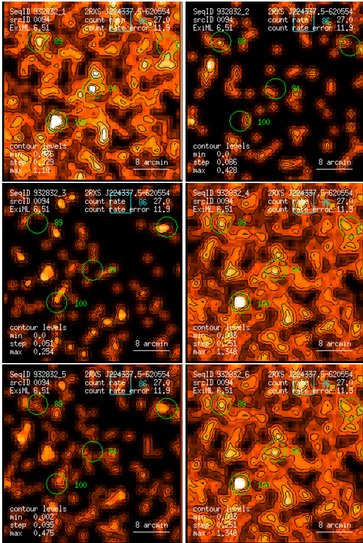
Figure 94: RASS 932832: detection 0094: band rate images, Gaussian filter: (1) PSPC channels 11 – 41, (2) 52 – 90, (3) 91 – 201, (4) 11 – 235, (5) 52 – 201, (6) 11 – 201. Broad band rates in counts/ks. Band rate contour levels in counts/ks/arcmin 2 .
