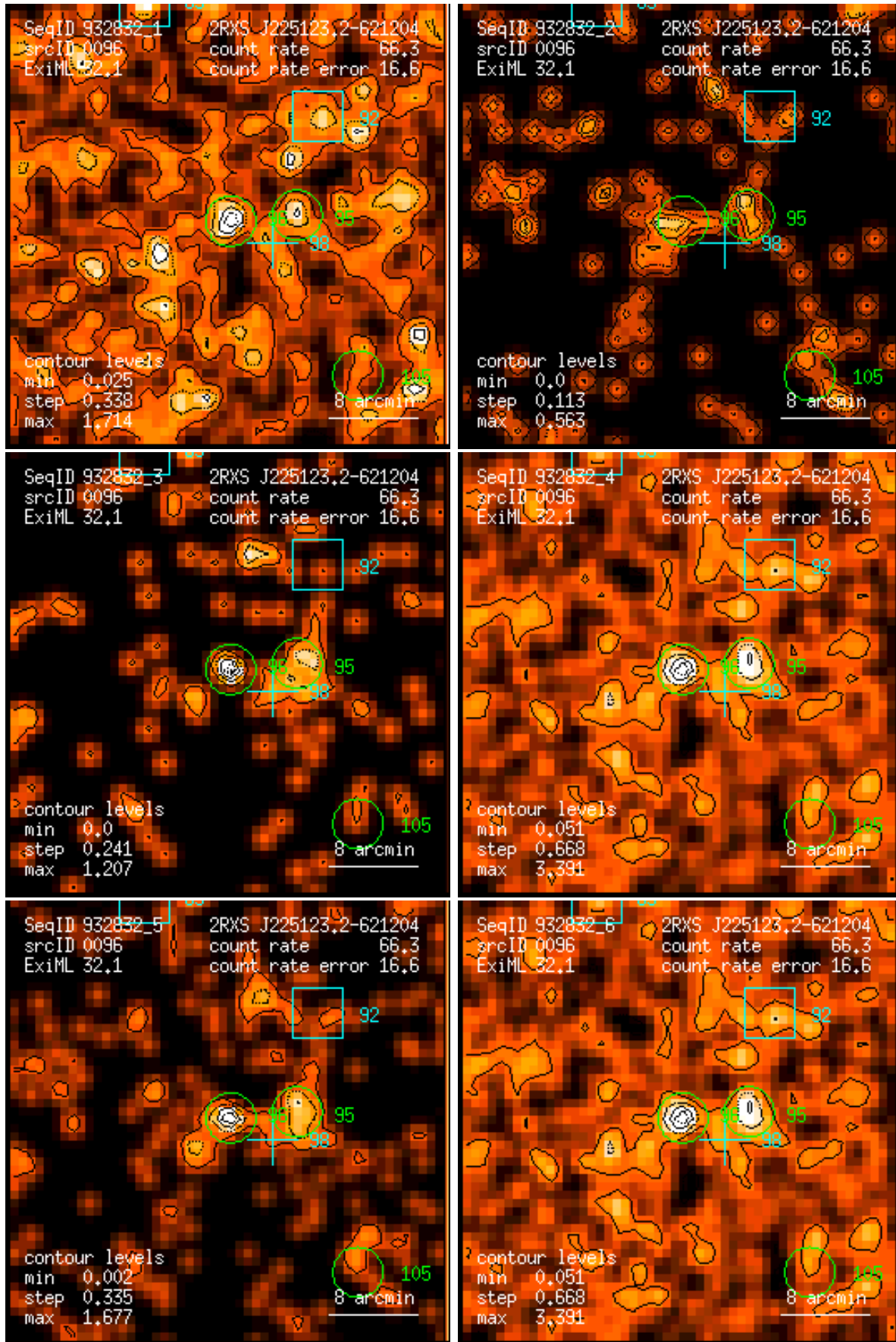
Figure 96: RASS 932832: detection 0096: band rate images, Gaussian filter: (1) PSPC channels 11 – 41, (2) 52 – 90, (3) 91 – 201, (4) 11 – 235, (5) 52 – 201, (6) 11 – 201. Broad band rates in counts/ks. Band rate contour levels in counts/ks/arcmin 2 .
