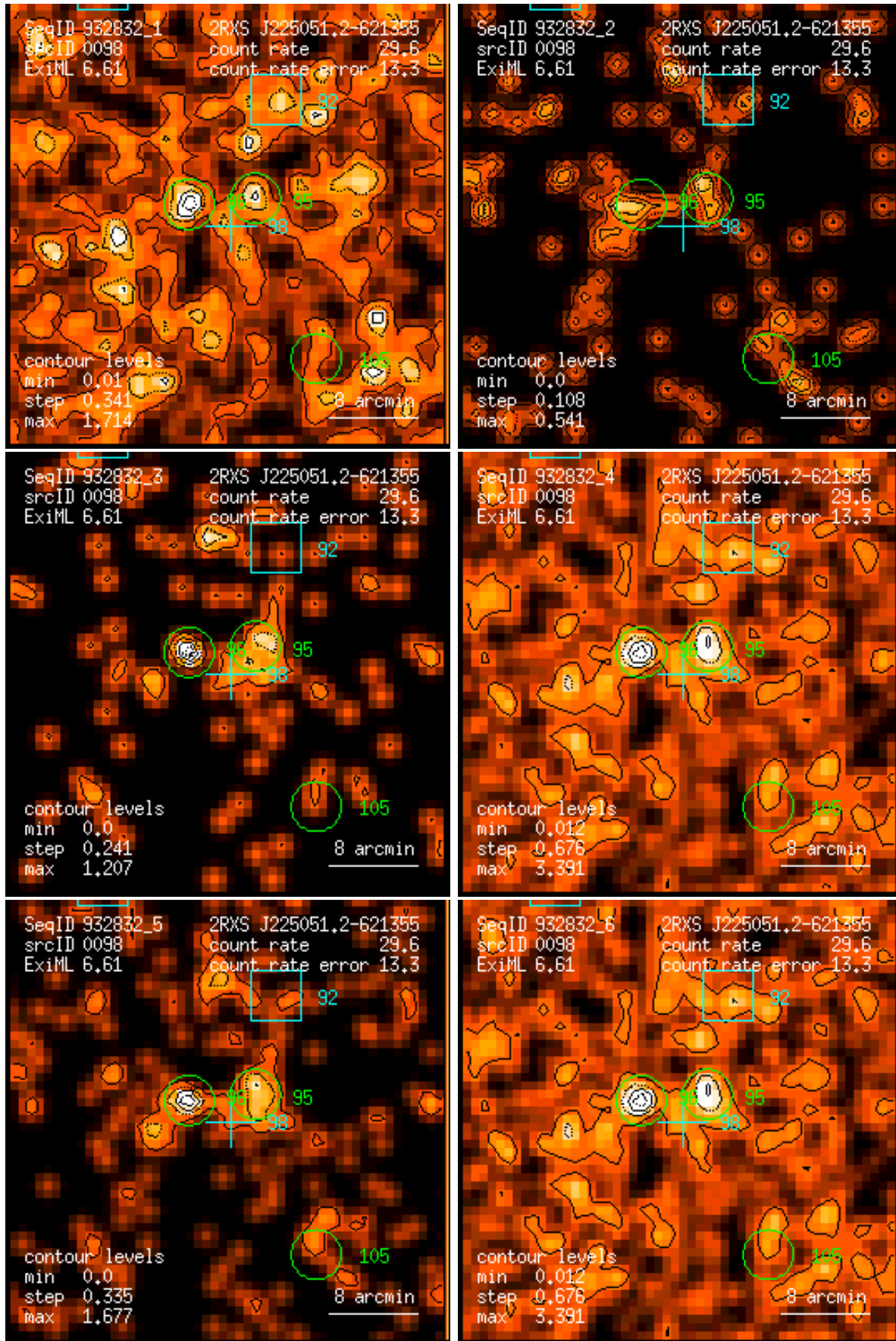
Figure 98: RASS 932832: detection 0098: band rate images, Gaussian filter: (1) PSPC channels 11 – 41, (2) 52 – 90, (3) 91 – 201, (4) 11 – 235, (5) 52 – 201, (6) 11 – 201. Broad band rates in counts/ks. Band rate contour levels in counts/ks/arcmin 2 .
