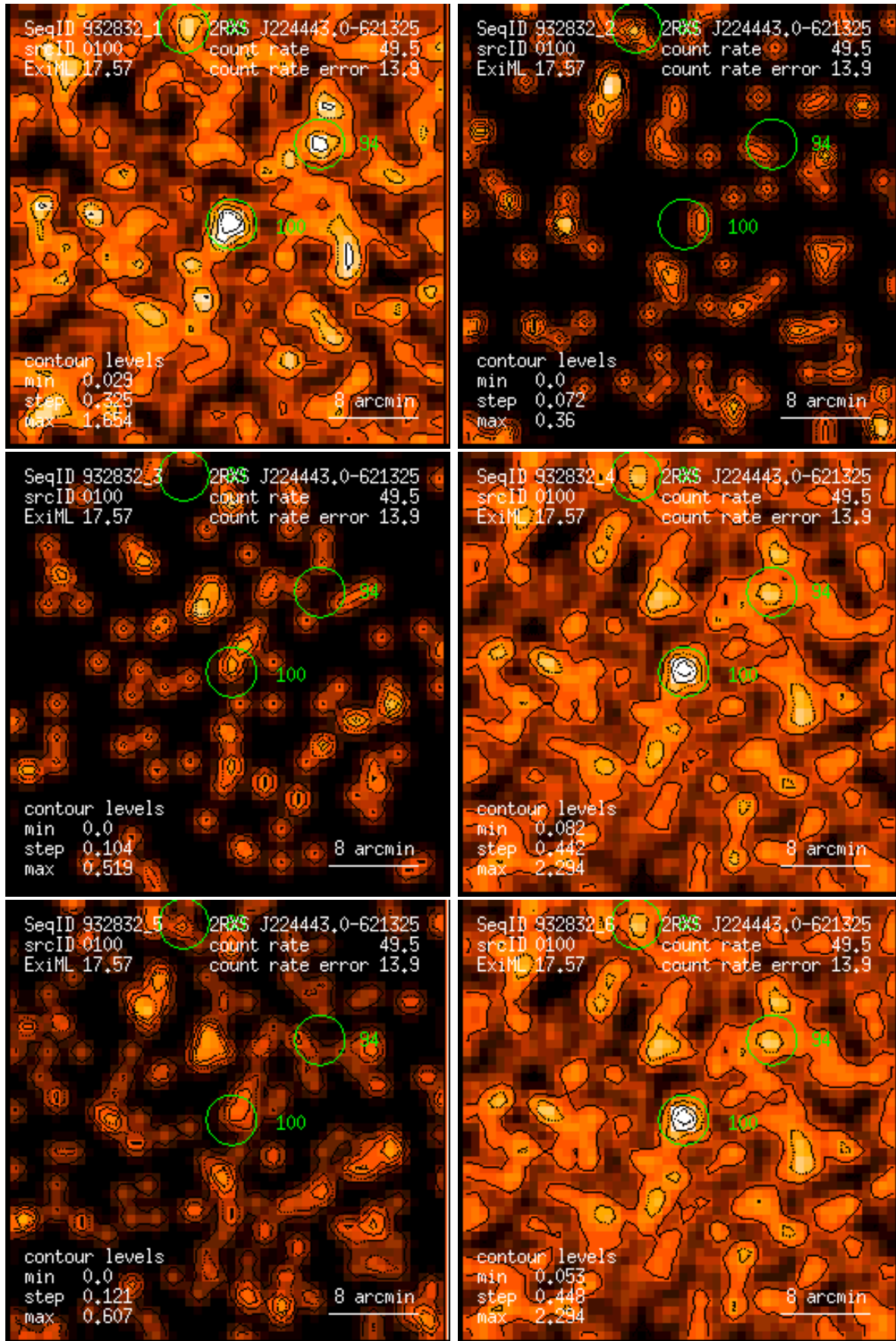
Figure 100: RASS 932832: detection 0100: band rate images, Gaussian filter: (1) PSPC channels 11 – 41, (2) 52 – 90, (3) 91 – 201, (4) 11 – 235, (5) 52 – 201, (6) 11 – 201. Broad band rates in counts/ks. Band rate contour levels in counts/ks/arcmin 2 .
