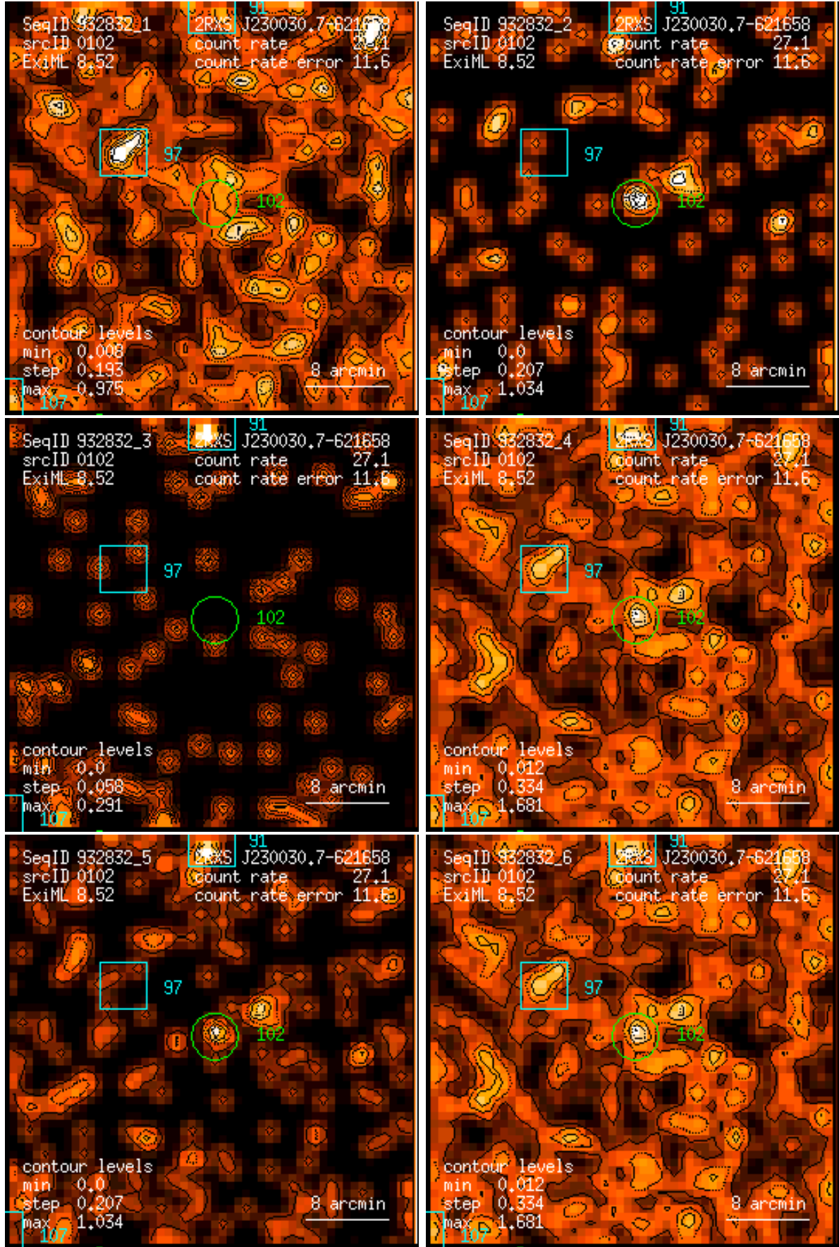
Figure 102: RASS 932832: detection 0102: band rate images, Gaussian filter: (1) PSPC channels 11 – 41, (2) 52 – 90, (3) 91 – 201, (4) 11 – 235, (5) 52 – 201, (6) 11 – 201. Broad band rates in counts/ks. Band rate contour levels in counts/ks/arcmin 2 .
