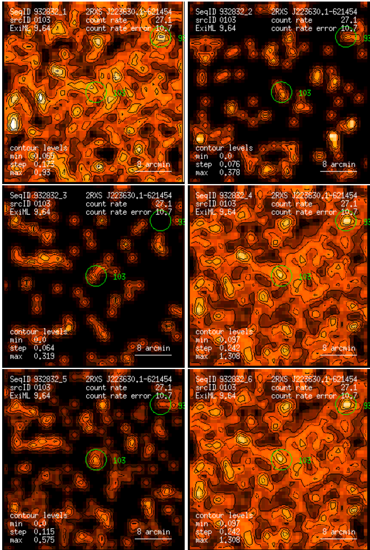
Figure 103: RASS 932832: detection 0103: band rate images, Gaussian filter: (1) PSPC channels 11 – 41, (2) 52 – 90, (3) 91 – 201, (4) 11 – 235, (5) 52 – 201, (6) 11 – 201. Broad band rates in counts/ks. Band rate contour levels in counts/ks/arcmin 2 .
