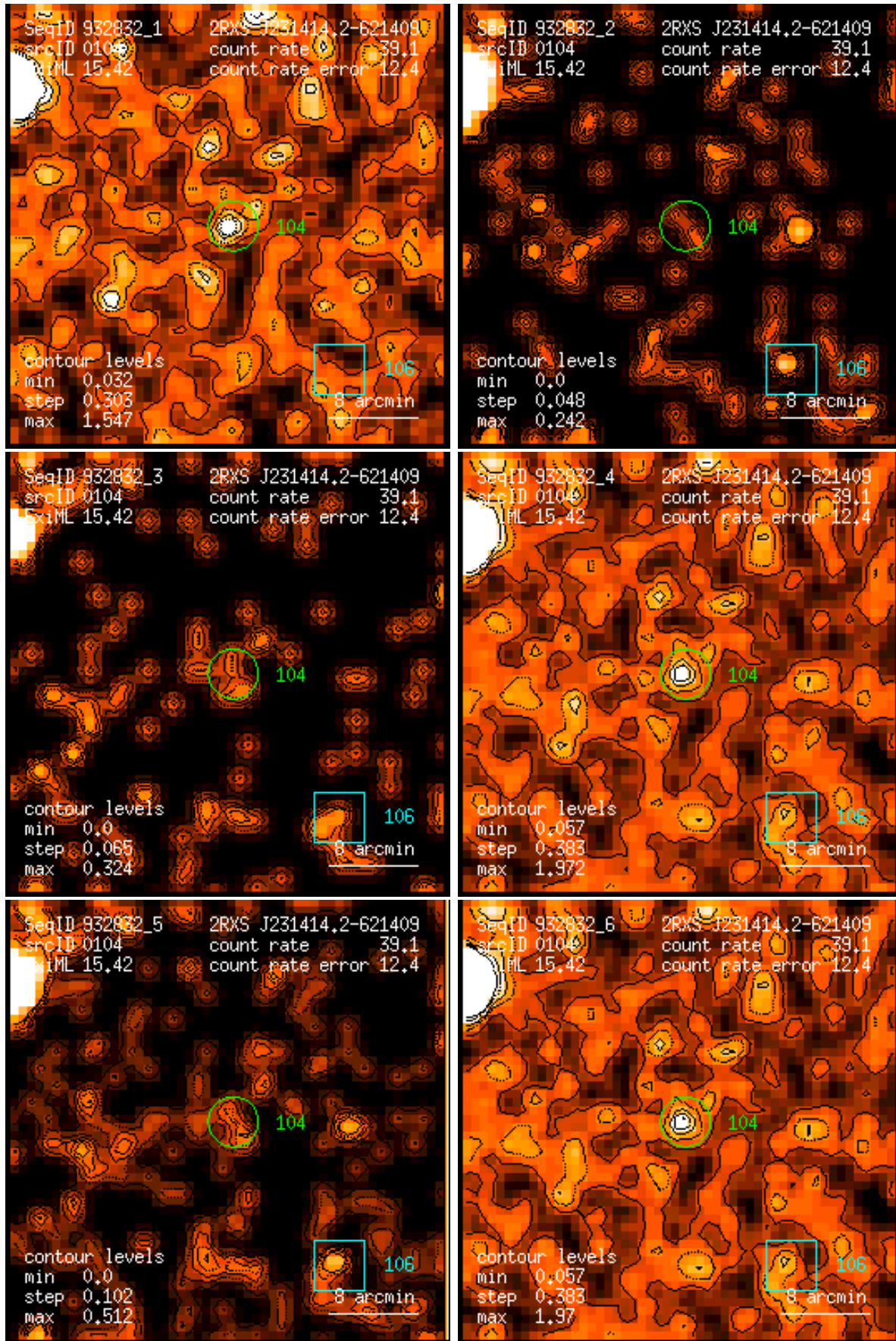
Figure 104: RASS 932832: detection 0104: band rate images, Gaussian filter: (1) PSPC channels 11 – 41, (2) 52 – 90, (3) 91 – 201, (4) 11 – 235, (5) 52 – 201, (6) 11 – 201. Broad band rates in counts/ks. Band rate contour levels in counts/ks/arcmin 2 .
