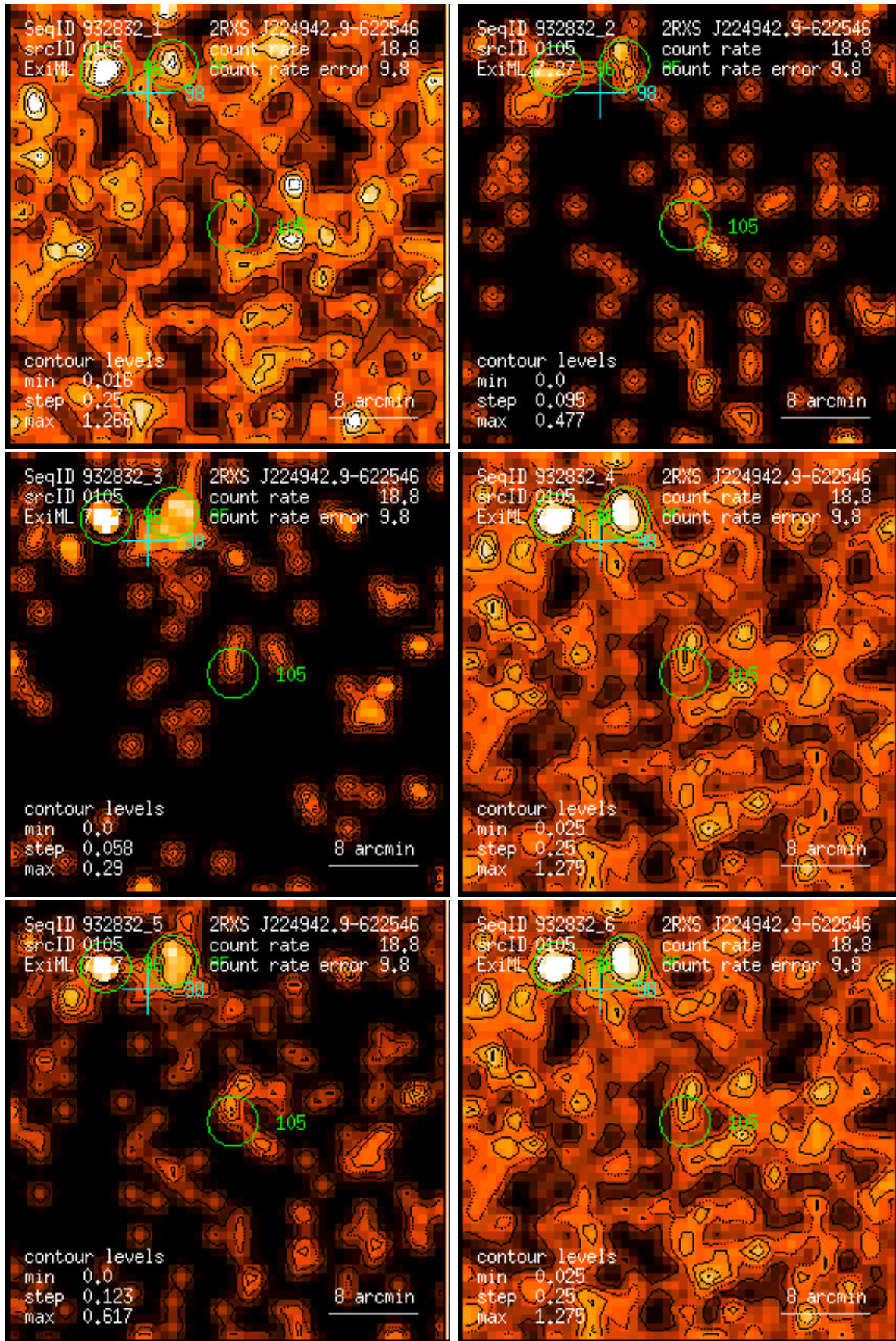
Figure 105: RASS 932832: detection 0105: band rate images, Gaussian filter: (1) PSPC channels 11 – 41, (2) 52 – 90, (3) 91 – 201, (4) 11 – 235, (5) 52 – 201, (6) 11 – 201. Broad band rates in counts/ks. Band rate contour levels in counts/ks/arcmin 2 .
