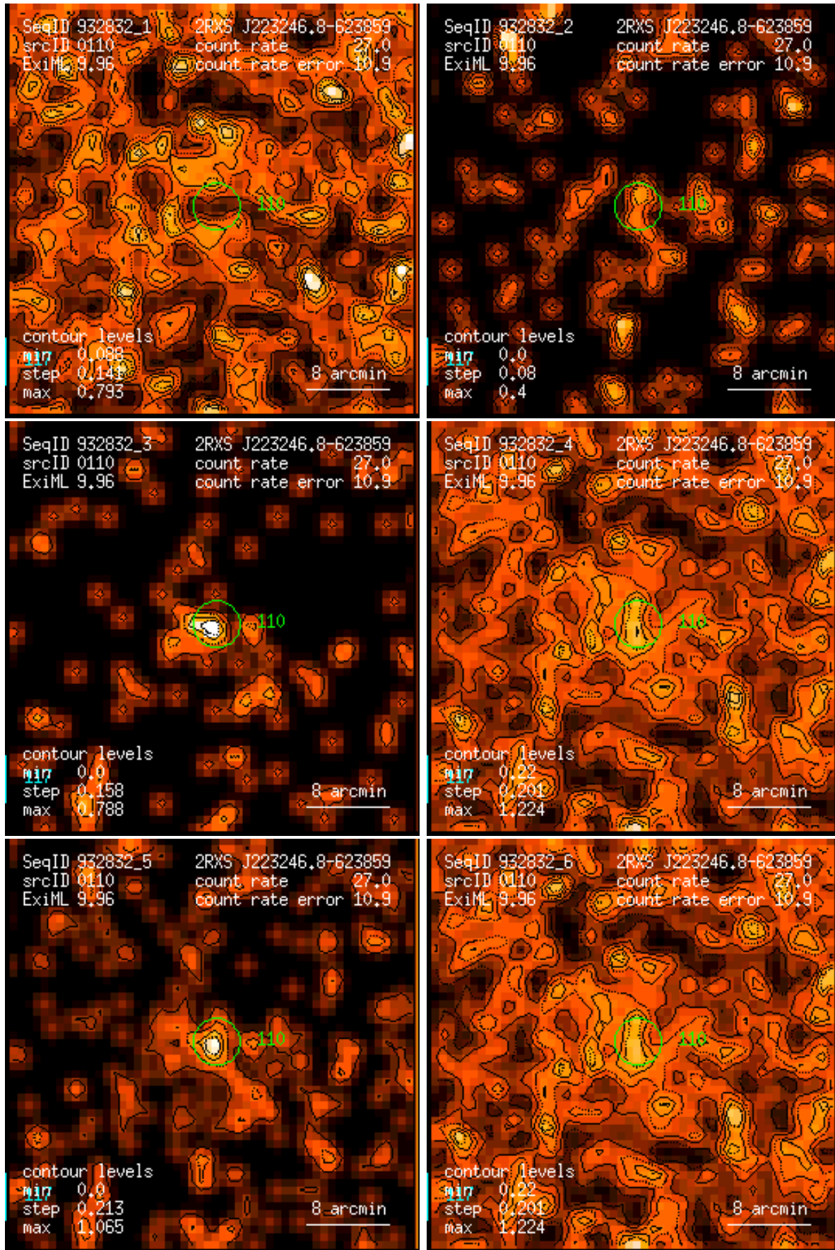
Figure 110: RASS 932832: detection 0110: band rate images, Gaussian filter: (1) PSPC channels 11 – 41, (2) 52 – 90, (3) 91 – 201, (4) 11 – 235, (5) 52 – 201, (6) 11 – 201. Broad band rates in counts/ks. Band rate contour levels in counts/ks/arcmin 2 .
