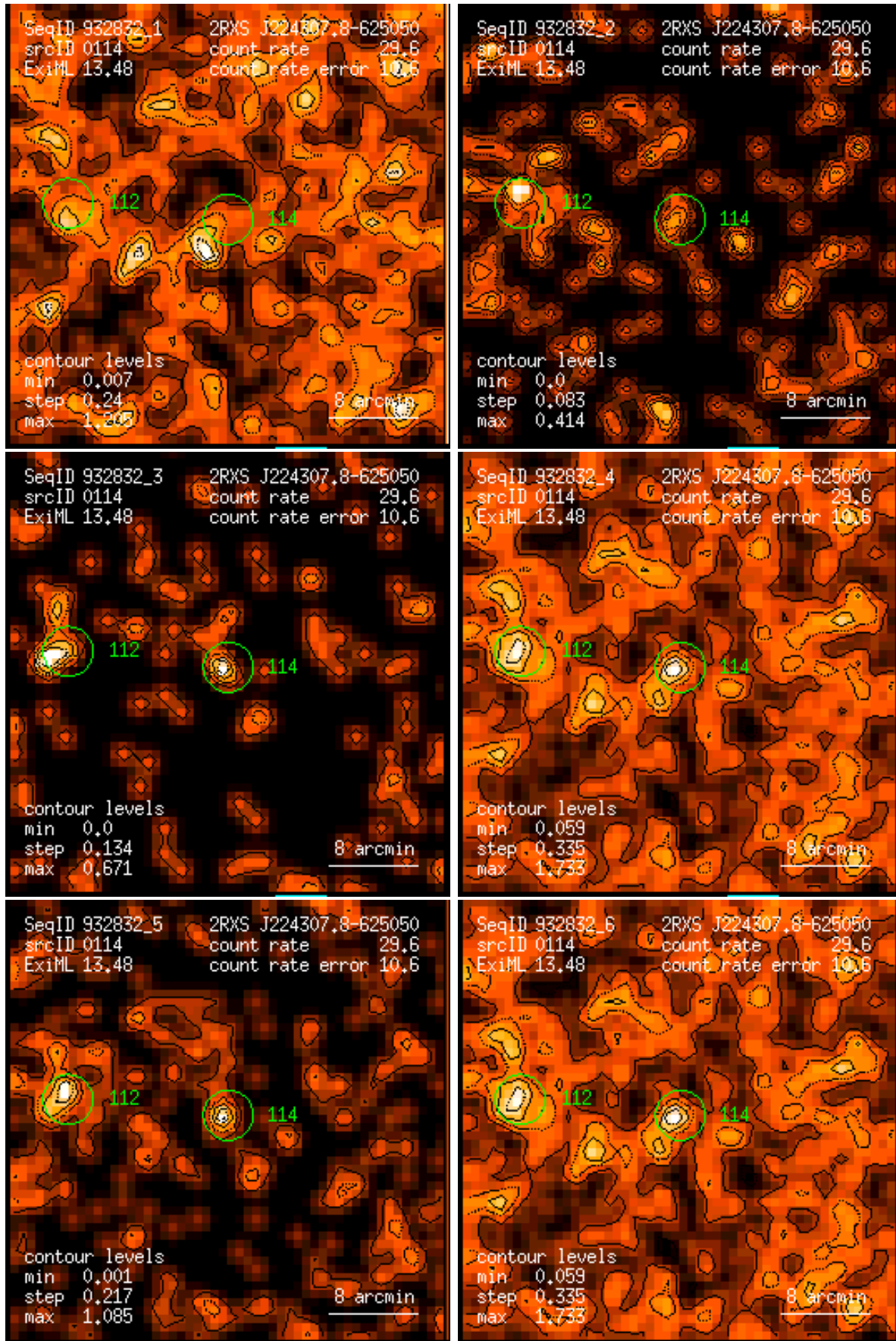
Figure 114: RASS 932832: detection 0114: band rate images, Gaussian filter: (1) PSPC channels 11 – 41, (2) 52 – 90, (3) 91 – 201, (4) 11 – 235, (5) 52 – 201, (6) 11 – 201. Broad band rates in counts/ks. Band rate contour levels in counts/ks/arcmin 2 .
