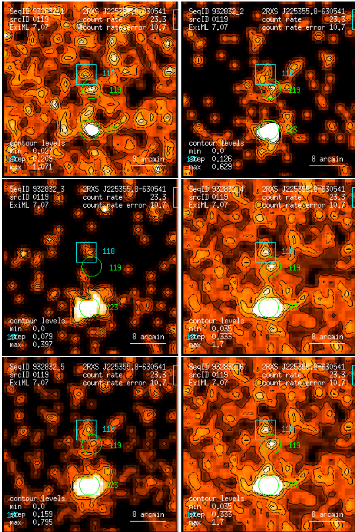
Figure 119: RASS 932832: detection 0119: band rate images, Gaussian filter: (1) PSPC channels 11 – 41, (2) 52 – 90, (3) 91 – 201, (4) 11 – 235, (5) 52 – 201, (6) 11 – 201. Broad band rates in counts/ks. Band rate contour levels in counts/ks/arcmin 2 .
