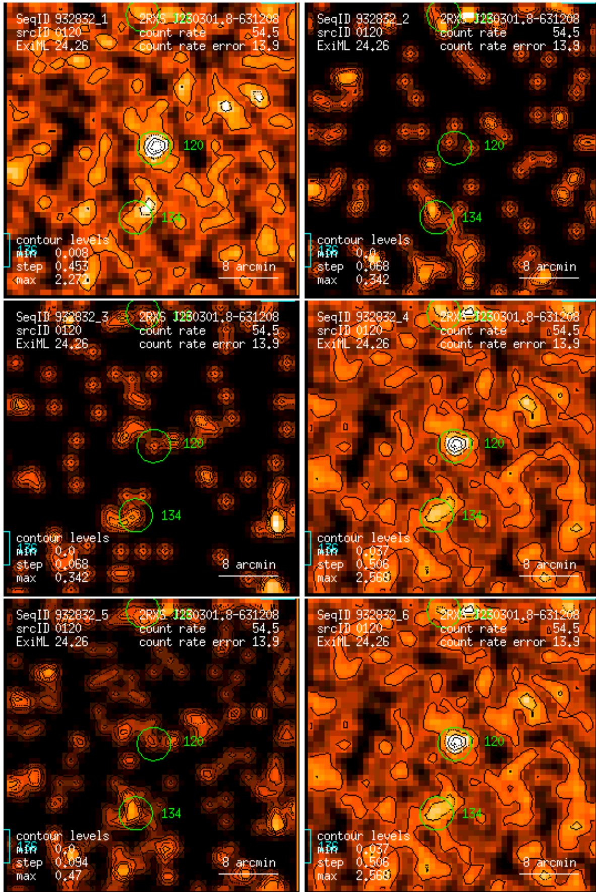
Figure 120: RASS 932832: detection 0120: band rate images, Gaussian filter: (1) PSPC channels 11 – 41, (2) 52 – 90, (3) 91 – 201, (4) 11 – 235, (5) 52 – 201, (6) 11 – 201. Broad band rates in counts/ks. Band rate contour levels in counts/ks/arcmin 2 .
