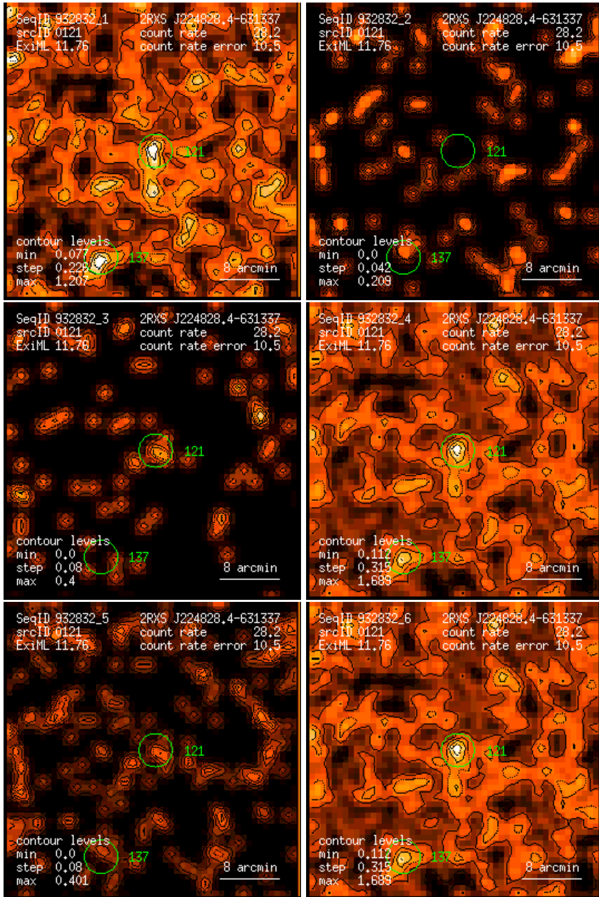
Figure 121: RASS 932832: detection 0121: band rate images, Gaussian filter: (1) PSPC channels 11 – 41, (2) 52 – 90, (3) 91 – 201, (4) 11 – 235, (5) 52 – 201, (6) 11 – 201. Broad band rates in counts/ks. Band rate contour levels in counts/ks/arcmin 2 .
