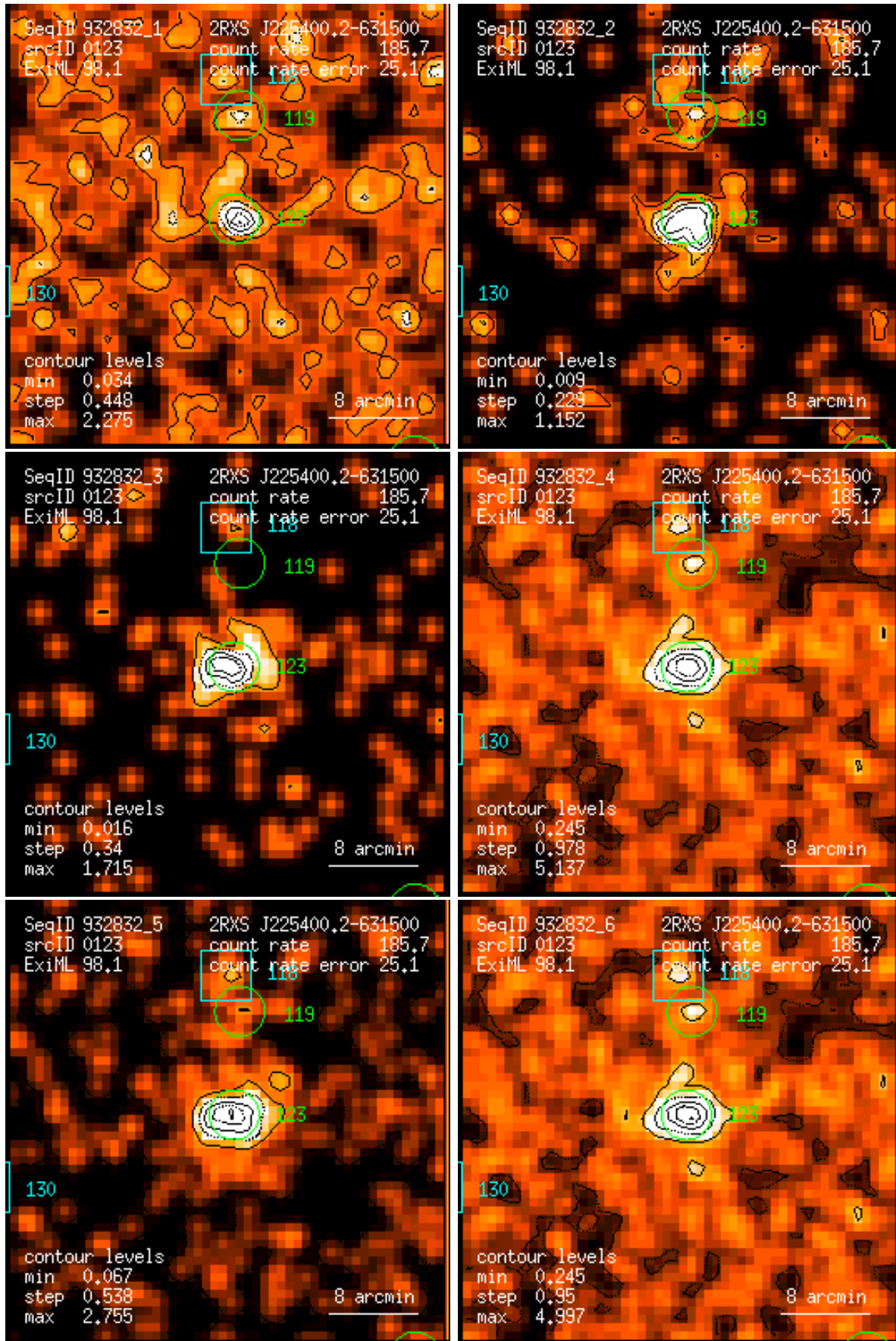
Figure 123: RASS 932832: detection 0123: band rate images, Gaussian filter: (1) PSPC channels 11 – 41, (2) 52 – 90, (3) 91 – 201, (4) 11 – 235, (5) 52 – 201, (6) 11 – 201. Broad band rates in counts/ks. Band rate contour levels in counts/ks/arcmin 2 .
