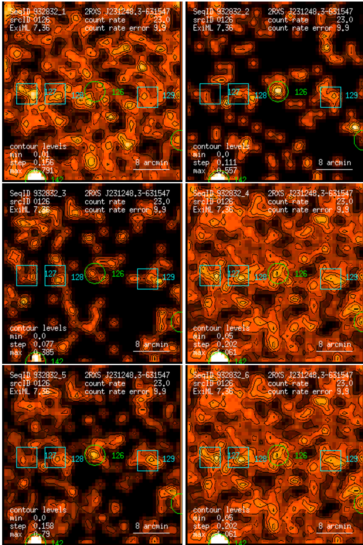
Figure 126: RASS 932832: detection 0126: band rate images, Gaussian filter: (1) PSPC channels 11 – 41, (2) 52 – 90, (3) 91 – 201, (4) 11 – 235, (5) 52 – 201, (6) 11 – 201. Broad band rates in counts/ks. Band rate contour levels in counts/ks/arcmin 2 .
