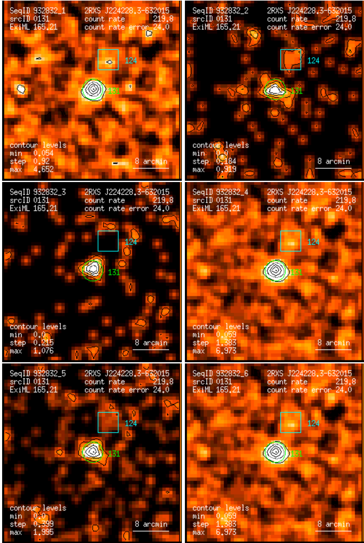
Figure 131: RASS 932832: detection 0131: band rate images, Gaussian filter: (1) PSPC channels 11 – 41, (2) 52 – 90, (3) 91 – 201, (4) 11 – 235, (5) 52 – 201, (6) 11 – 201. Broad band rates in counts/ks. Band rate contour levels in counts/ks/arcmin 2 .
