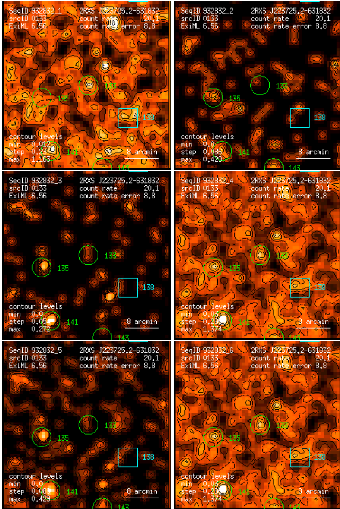
Figure 133: RASS 932832: detection 0133: band rate images, Gaussian filter: (1) PSPC channels 11 – 41, (2) 52 – 90, (3) 91 – 201, (4) 11 – 235, (5) 52 – 201, (6) 11 – 201. Broad band rates in counts/ks. Band rate contour levels in counts/ks/arcmin 2 .
