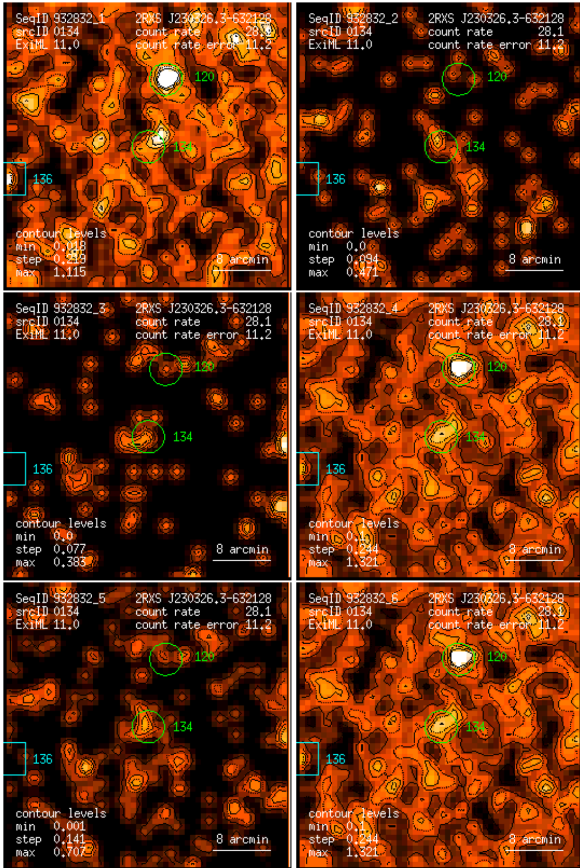
Figure 134: RASS 932832: detection 0134: band rate images, Gaussian filter: (1) PSPC channels 11 – 41, (2) 52 – 90, (3) 91 – 201, (4) 11 – 235, (5) 52 – 201, (6) 11 – 201. Broad band rates in counts/ks. Band rate contour levels in counts/ks/arcmin 2 .
