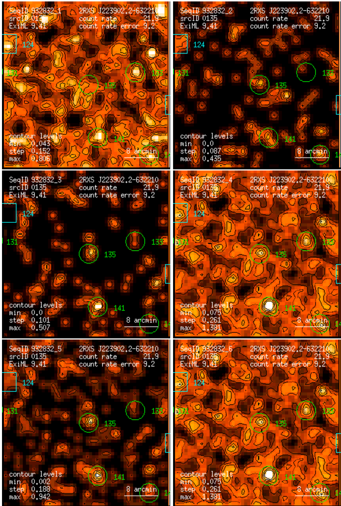
Figure 135: RASS 932832: detection 0135: band rate images, Gaussian filter: (1) PSPC channels 11 – 41, (2) 52 – 90, (3) 91 – 201, (4) 11 – 235, (5) 52 – 201, (6) 11 – 201. Broad band rates in counts/ks. Band rate contour levels in counts/ks/arcmin 2 .
