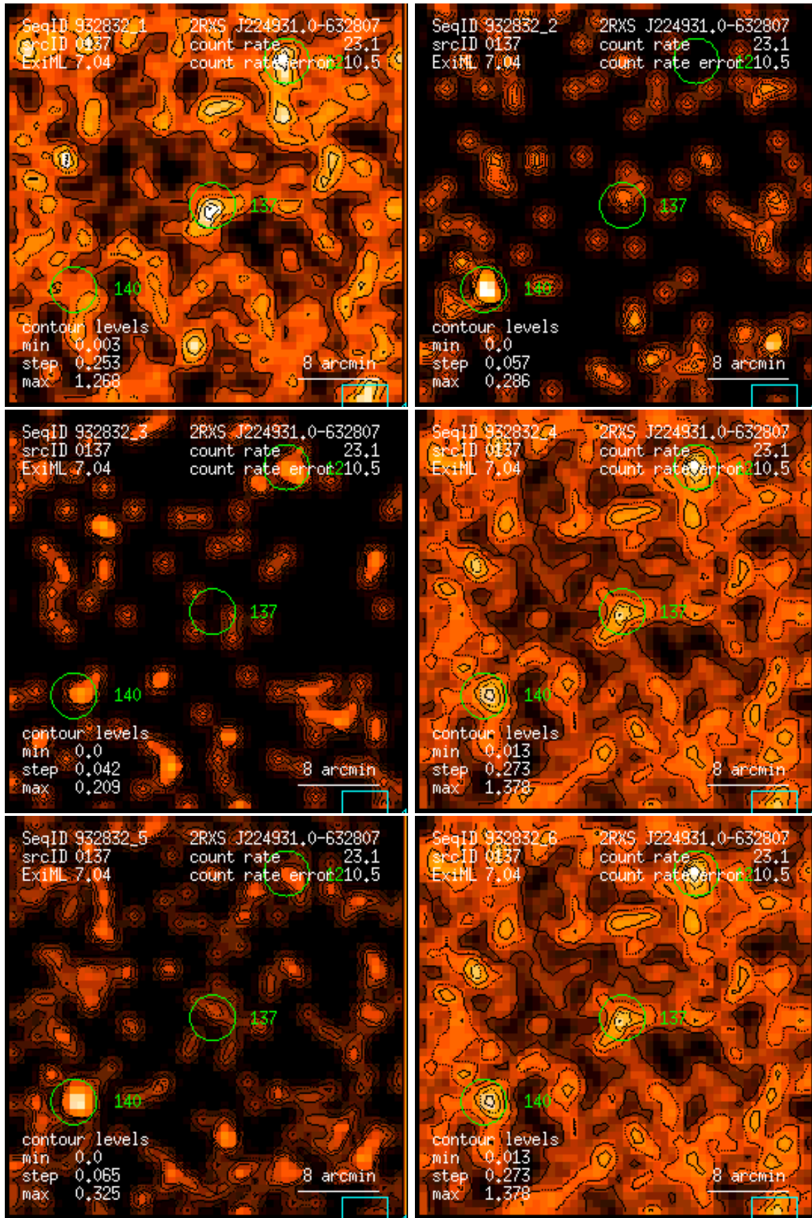
Figure 137: RASS 932832: detection 0137: band rate images, Gaussian filter: (1) PSPC channels 11 – 41, (2) 52 – 90, (3) 91 – 201, (4) 11 – 235, (5) 52 – 201, (6) 11 – 201. Broad band rates in counts/ks. Band rate contour levels in counts/ks/arcmin 2 .
