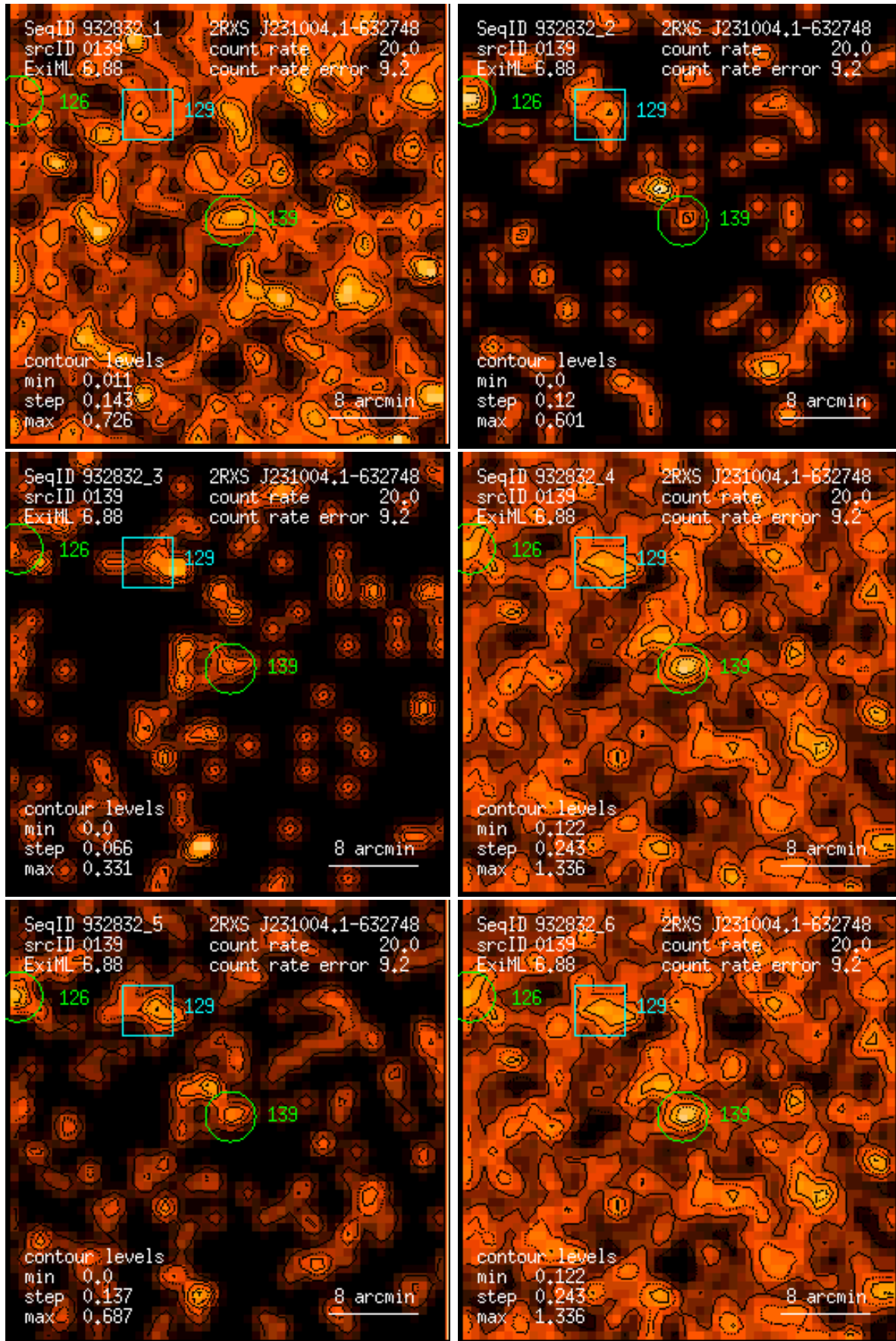
Figure 139: RASS 932832: detection 0139: band rate images, Gaussian filter: (1) PSPC channels 11 – 41, (2) 52 – 90, (3) 91 – 201, (4) 11 – 235, (5) 52 – 201, (6) 11 – 201. Broad band rates in counts/ks. Band rate contour levels in counts/ks/arcmin 2 .
