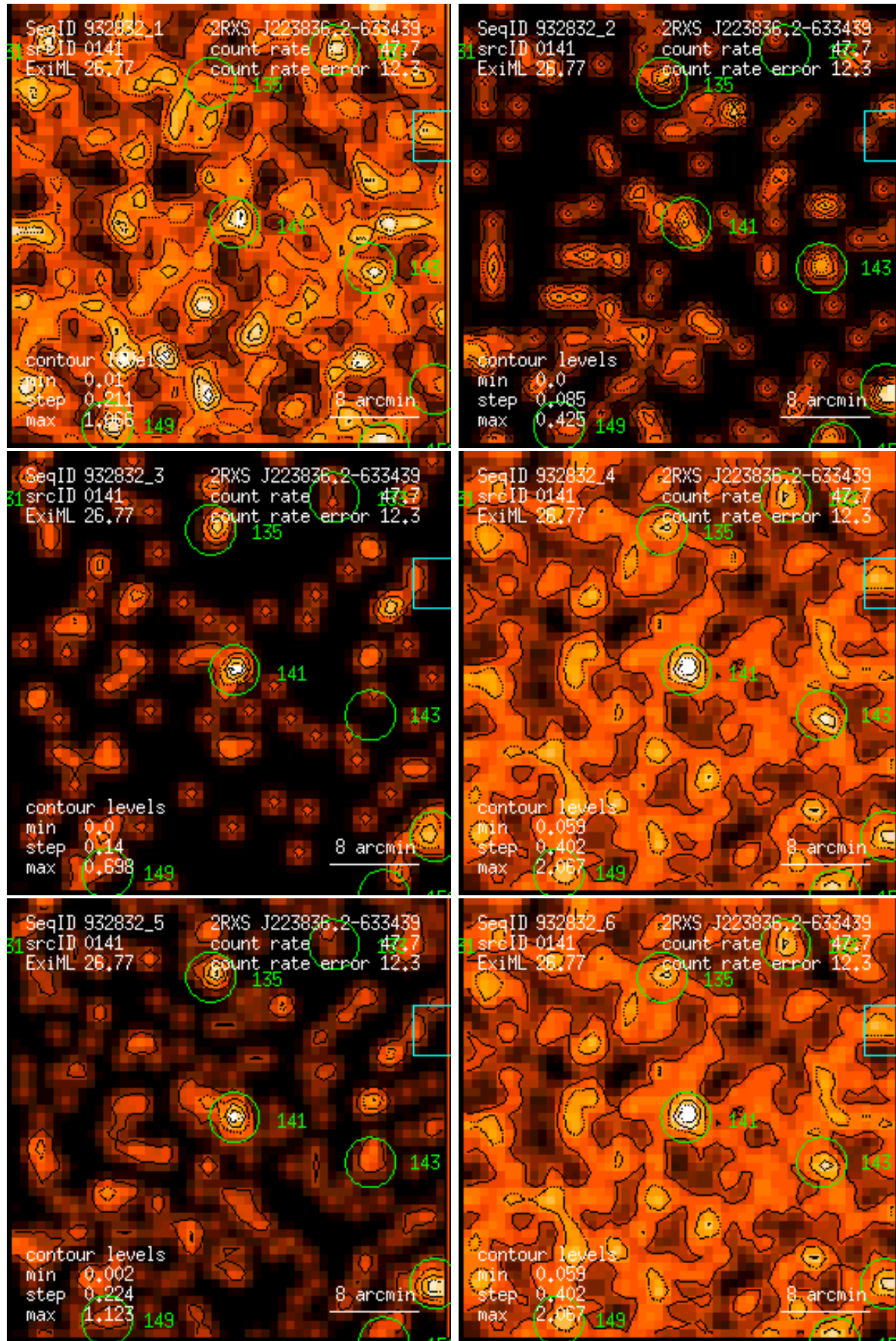
Figure 141: RASS 932832: detection 0141: band rate images, Gaussian filter: (1) PSPC channels 11 – 41, (2) 52 – 90, (3) 91 – 201, (4) 11 – 235, (5) 52 – 201, (6) 11 – 201. Broad band rates in counts/ks. Band rate contour levels in counts/ks/arcmin 2 .
