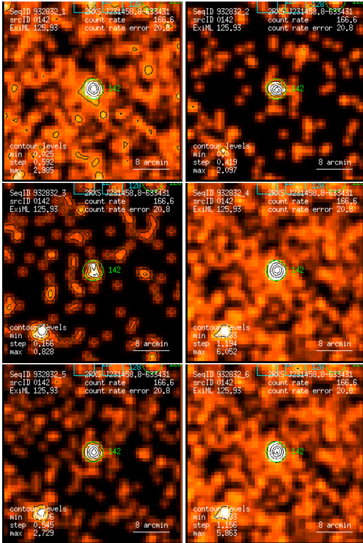
Figure 142: RASS 932832: detection 0142: band rate images, Gaussian filter: (1) PSPC channels 11 – 41, (2) 52 – 90, (3) 91 – 201, (4) 11 – 235, (5) 52 – 201, (6) 11 – 201. Broad band rates in counts/ks. Band rate contour levels in counts/ks/arcmin 2 .
