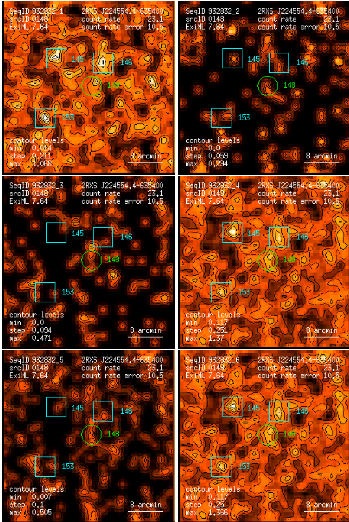
Figure 148: RASS 932832: detection 0148: band rate images, Gaussian filter: (1) PSPC channels 11 – 41, (2) 52 – 90, (3) 91 – 201, (4) 11 – 235, (5) 52 – 201, (6) 11 – 201. Broad band rates in counts/ks. Band rate contour levels in counts/ks/arcmin 2 .
