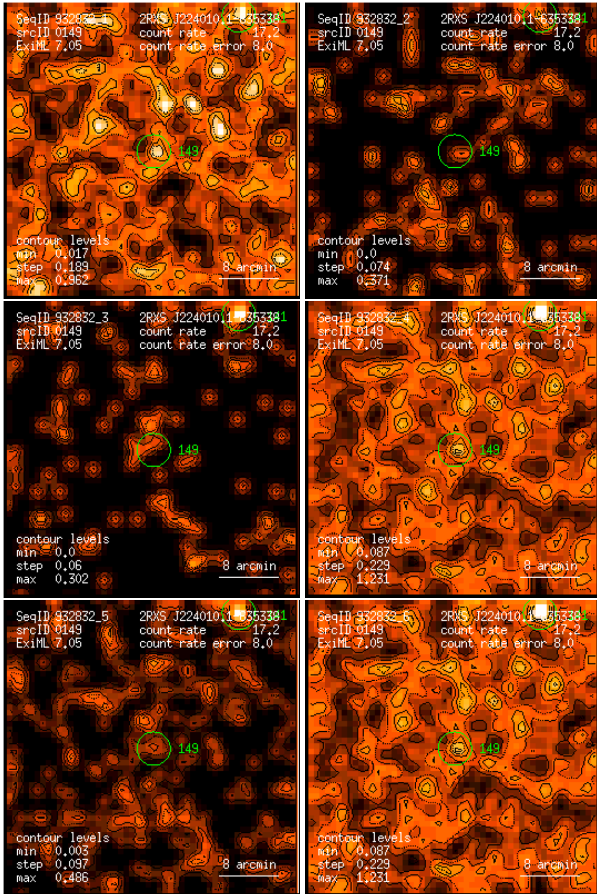
Figure 149: RASS 932832: detection 0149: band rate images, Gaussian filter: (1) PSPC channels 11 – 41, (2) 52 – 90, (3) 91 – 201, (4) 11 – 235, (5) 52 – 201, (6) 11 – 201. Broad band rates in counts/ks. Band rate contour levels in counts/ks/arcmin 2 .
