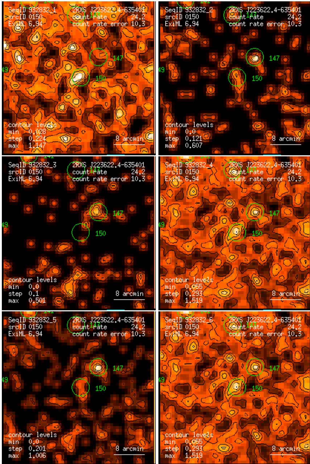
Figure 150: RASS 932832: detection 0150: band rate images, Gaussian filter: (1) PSPC channels 11 – 41, (2) 52 – 90, (3) 91 – 201, (4) 11 – 235, (5) 52 – 201, (6) 11 – 201. Broad band rates in counts/ks. Band rate contour levels in counts/ks/arcmin 2 .
