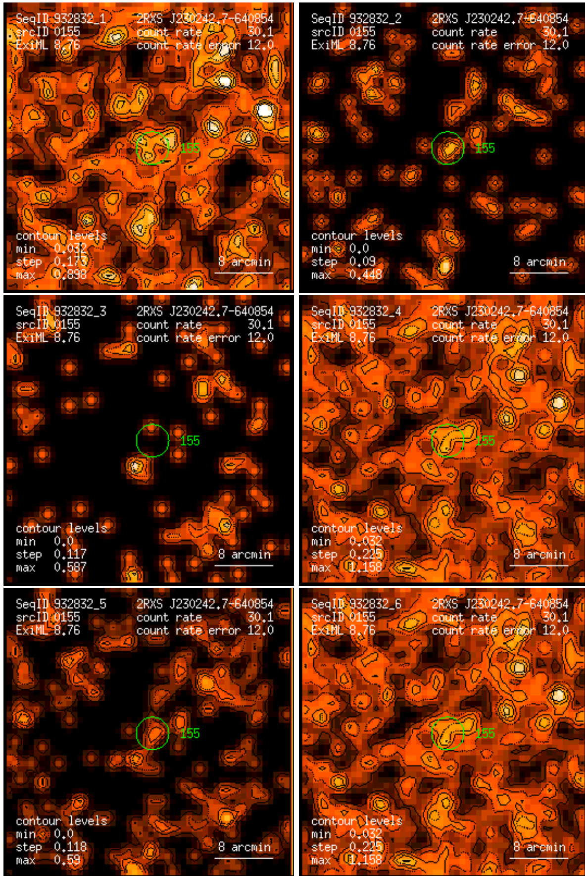
Figure 155: RASS 932832: detection 0155: band rate images, Gaussian filter: (1) PSPC channels 11 – 41, (2) 52 – 90, (3) 91 – 201, (4) 11 – 235, (5) 52 – 201, (6) 11 – 201. Broad band rates in counts/ks. Band rate contour levels in counts/ks/arcmin 2 .
