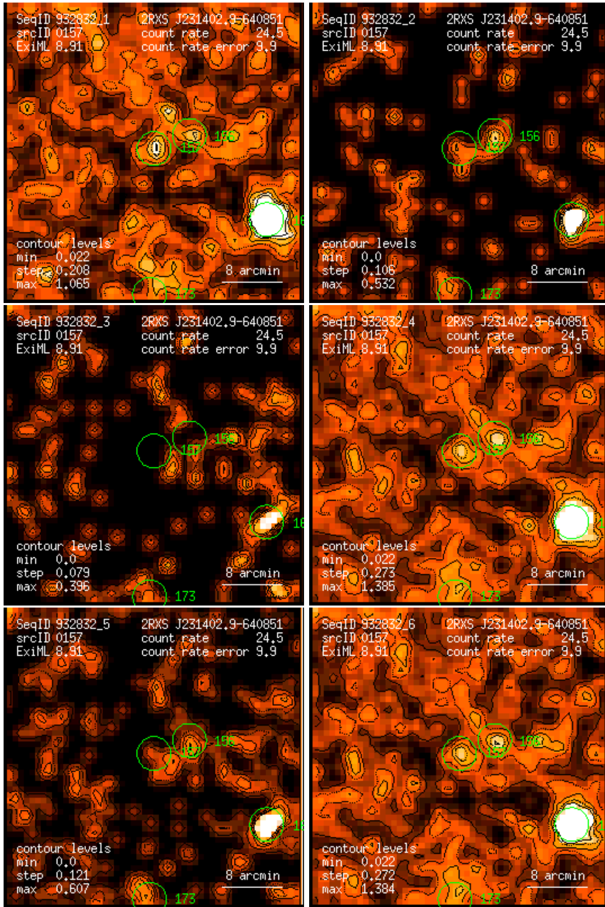
Figure 157: RASS 932832: detection 0157: band rate images, Gaussian filter: (1) PSPC channels 11 – 41, (2) 52 – 90, (3) 91 – 201, (4) 11 – 235, (5) 52 – 201, (6) 11 – 201. Broad band rates in counts/ks. Band rate contour levels in counts/ks/arcmin 2 .
