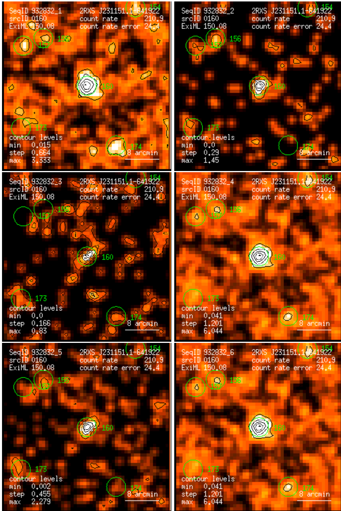
Figure 160: RASS 932832: detection 0160: band rate images, Gaussian filter: (1) PSPC channels 11 – 41, (2) 52 – 90, (3) 91 – 201, (4) 11 – 235, (5) 52 – 201, (6) 11 – 201. Broad band rates in counts/ks. Band rate contour levels in counts/ks/arcmin 2 .
