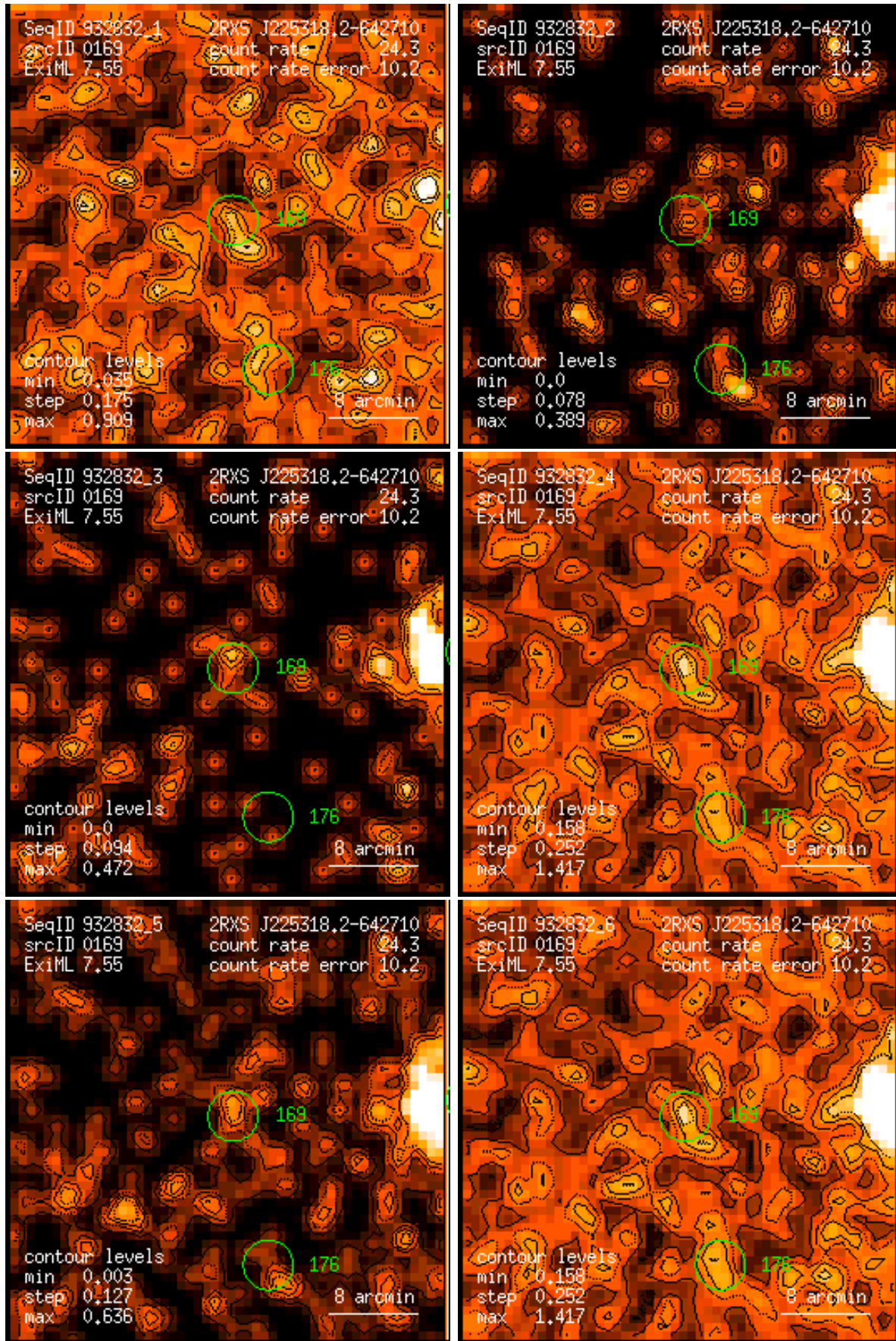
Figure 169: RASS 932832: detection 0169: band rate images, Gaussian filter: (1) PSPC channels 11 – 41, (2) 52 – 90, (3) 91 – 201, (4) 11 – 235, (5) 52 – 201, (6) 11 – 201. Broad band rates in counts/ks. Band rate contour levels in counts/ks/arcmin 2 .
