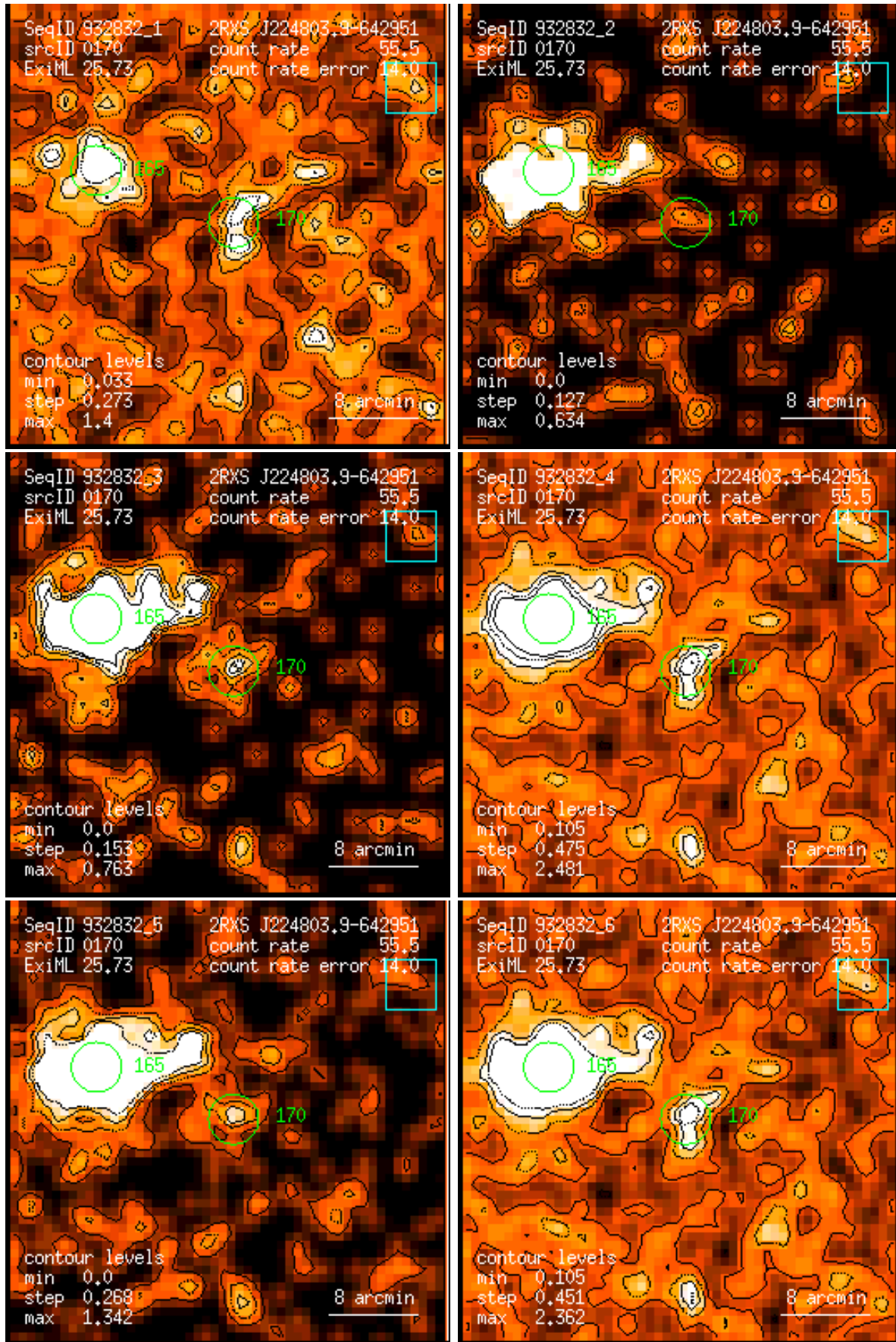
Figure 170: RASS 932832: detection 0170: band rate images, Gaussian filter: (1) PSPC channels 11 – 41, (2) 52 – 90, (3) 91 – 201, (4) 11 – 235, (5) 52 – 201, (6) 11 – 201. Broad band rates in counts/ks. Band rate contour levels in counts/ks/arcmin 2 .
