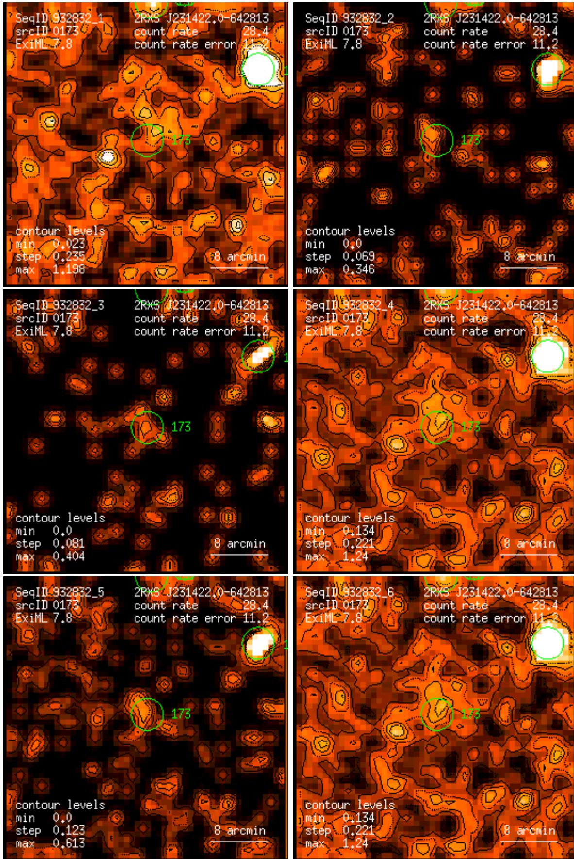
Figure 173: RASS 932832: detection 0173: band rate images, Gaussian filter: (1) PSPC channels 11 – 41, (2) 52 – 90, (3) 91 – 201, (4) 11 – 235, (5) 52 – 201, (6) 11 – 201. Broad band rates in counts/ks. Band rate contour levels in counts/ks/arcmin 2 .
