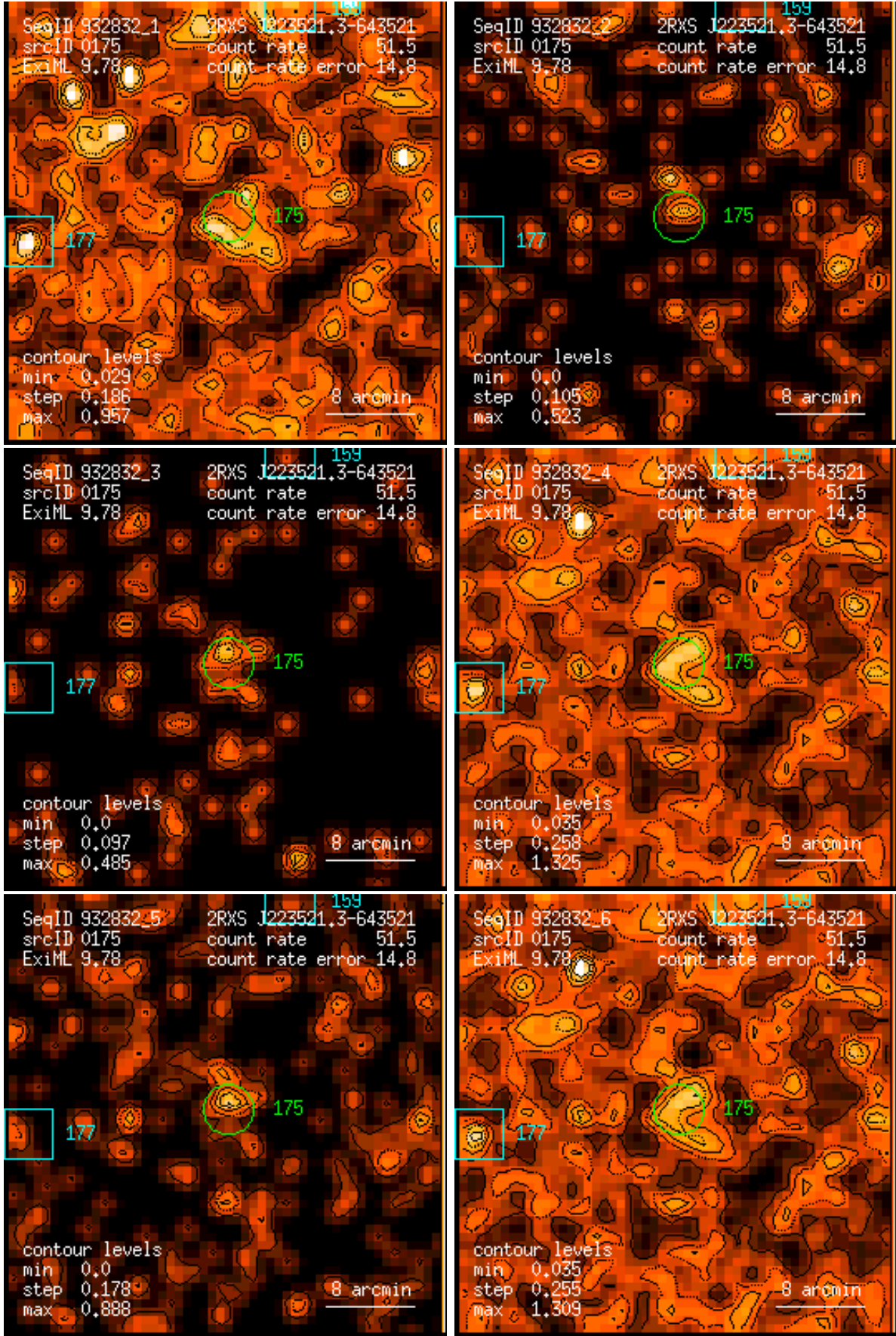
Figure 175: RASS 932832: detection 0175: band rate images, Gaussian filter: (1) PSPC channels 11 – 41, (2) 52 – 90, (3) 91 – 201, (4) 11 – 235, (5) 52 – 201, (6) 11 – 201. Broad band rates in counts/ks. Band rate contour levels in counts/ks/arcmin 2 .
