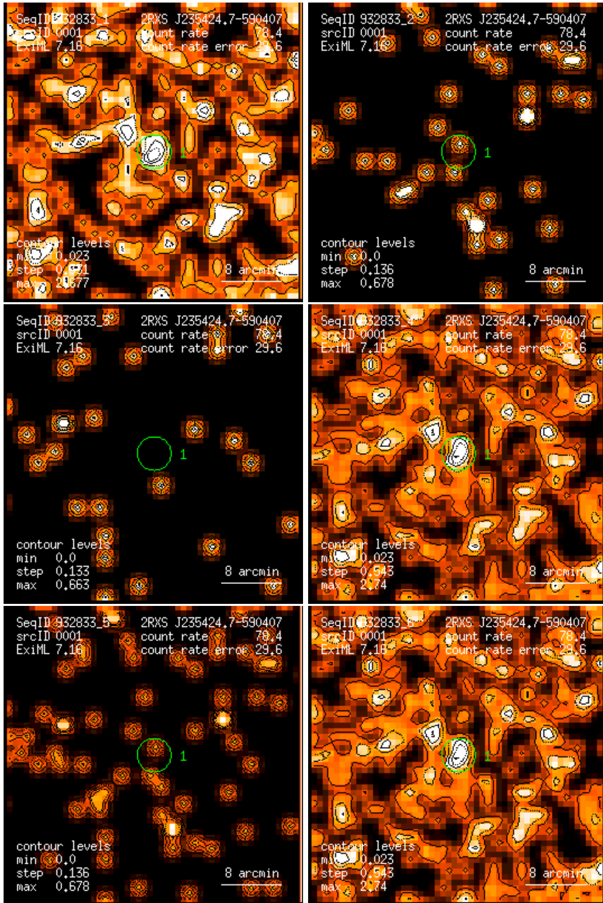
Figure 1: RASS 932833: detection 0001: band rate images, Gaussian filter: (1) PSPC channels 11 – 41, (2) 52 – 90, (3) 91 – 201, (4) 11 – 235, (5) 52 – 201, (6) 11 – 201. Broad band rates in counts/ks. Band rate contour levels in counts/ks/arcmin 2 .
