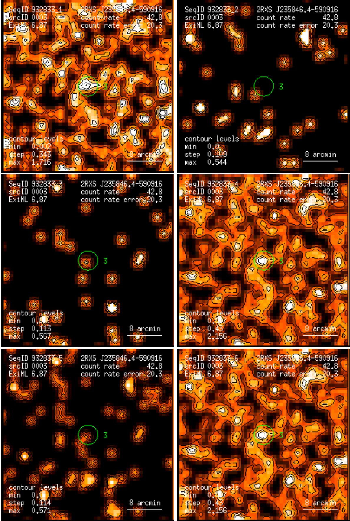
Figure 3: RASS 932833: detection 0003: band rate images, Gaussian filter: (1) PSPC channels 11 – 41, (2) 52 – 90, (3) 91 – 201, (4) 11 – 235, (5) 52 – 201, (6) 11 – 201. Broad band rates in counts/ks. Band rate contour levels in counts/ks/arcmin 2 .
