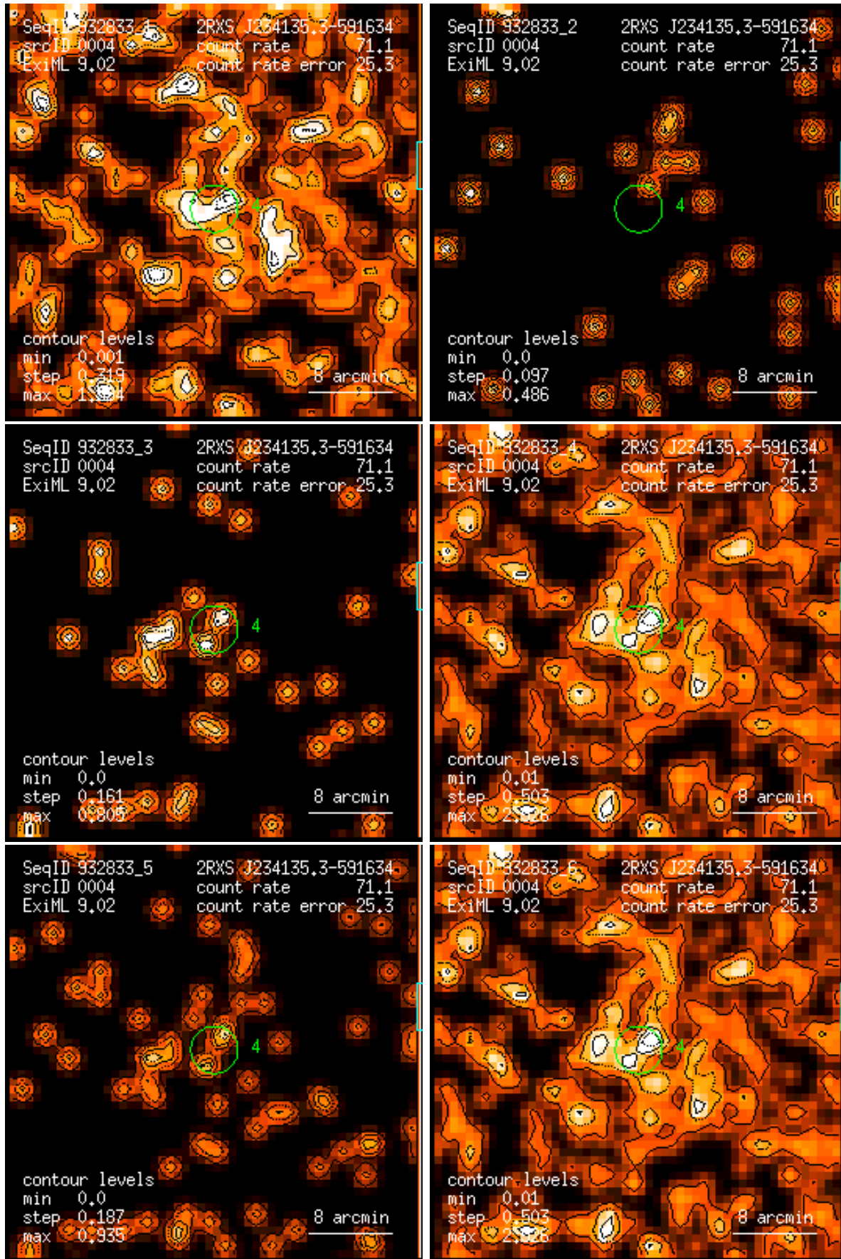
Figure 4: RASS 932833: detection 0004: band rate images, Gaussian filter: (1) PSPC channels 11 – 41, (2) 52 – 90, (3) 91 – 201, (4) 11 – 235, (5) 52 – 201, (6) 11 – 201. Broad band rates in counts/ks. Band rate contour levels in counts/ks/arcmin 2 .
