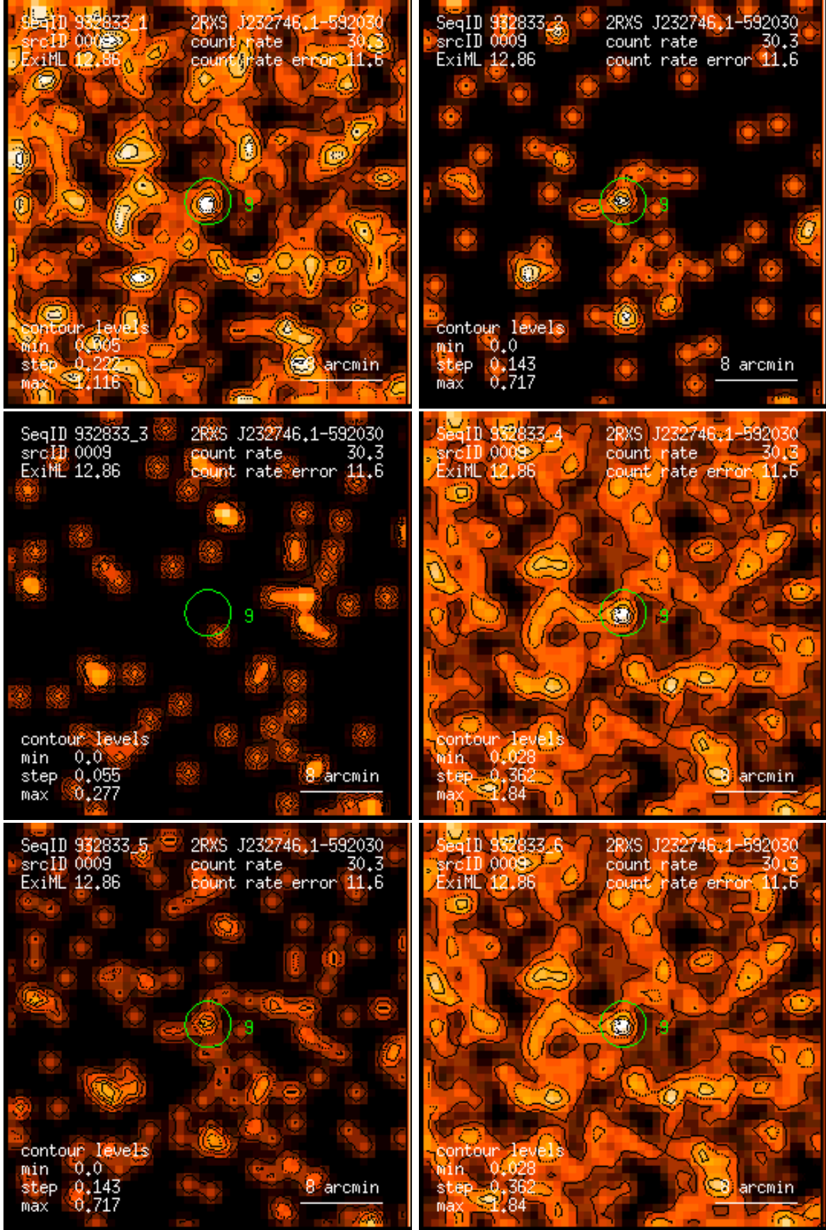
Figure 9: RASS 932833: detection 0009: band rate images, Gaussian filter: (1) PSPC channels 11 – 41, (2) 52 – 90, (3) 91 – 201, (4) 11 – 235, (5) 52 – 201, (6) 11 – 201. Broad band rates in counts/ks. Band rate contour levels in counts/ks/arcmin 2 .
