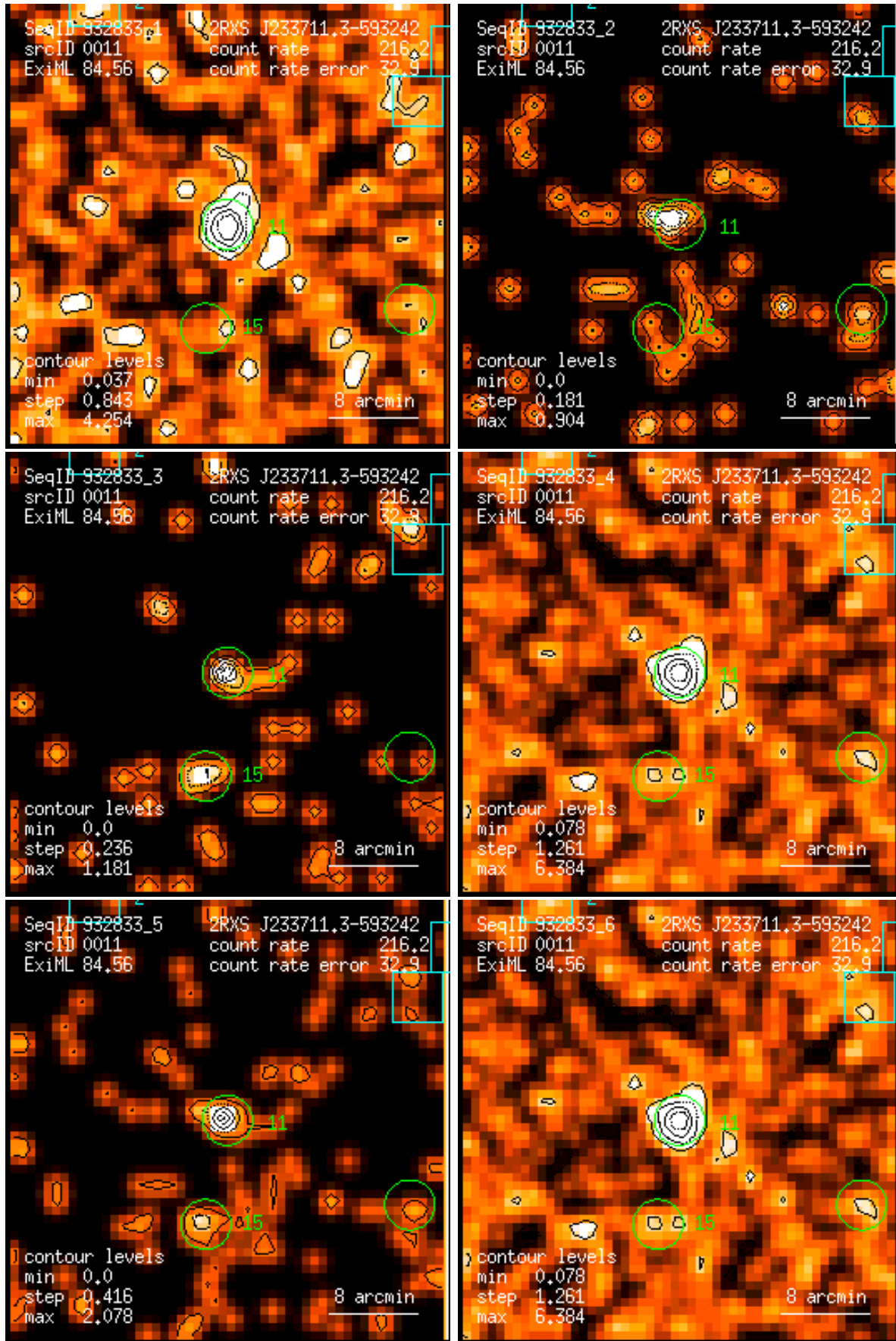
Figure 11: RASS 932833: detection 0011: band rate images, Gaussian filter: (1) PSPC channels 11 – 41, (2) 52 – 90, (3) 91 – 201, (4) 11 – 235, (5) 52 – 201, (6) 11 – 201. Broad band rates in counts/ks. Band rate contour levels in counts/ks/arcmin 2 .
