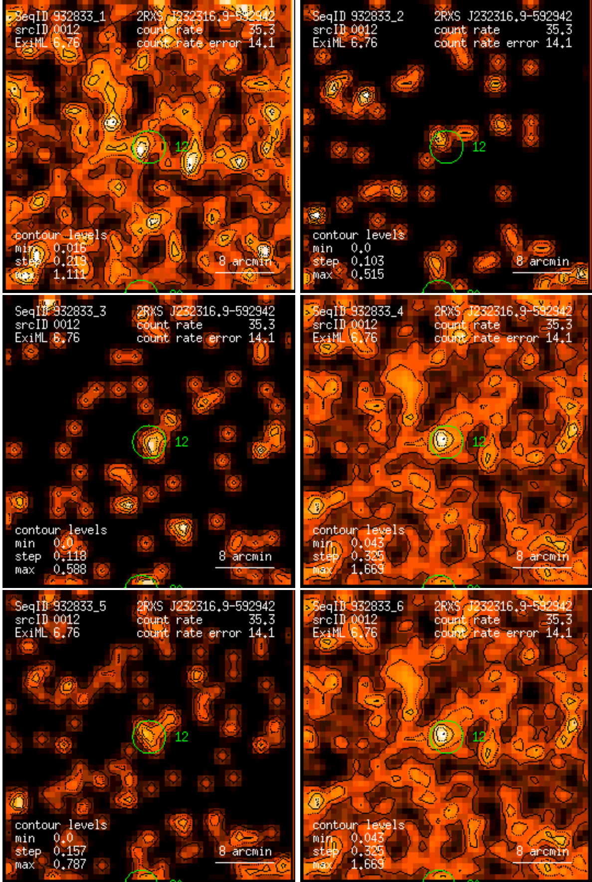
Figure 12: RASS 932833: detection 0012: band rate images, Gaussian filter: (1) PSPC channels 11 – 41, (2) 52 – 90, (3) 91 – 201, (4) 11 – 235, (5) 52 – 201, (6) 11 – 201. Broad band rates in counts/ks. Band rate contour levels in counts/ks/arcmin 2 .
