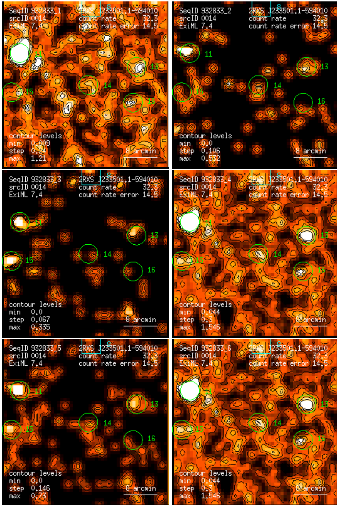
Figure 14: RASS 932833: detection 0014: band rate images, Gaussian filter: (1) PSPC channels 11 – 41, (2) 52 – 90, (3) 91 – 201, (4) 11 – 235, (5) 52 – 201, (6) 11 – 201. Broad band rates in counts/ks. Band rate contour levels in counts/ks/arcmin 2 .
