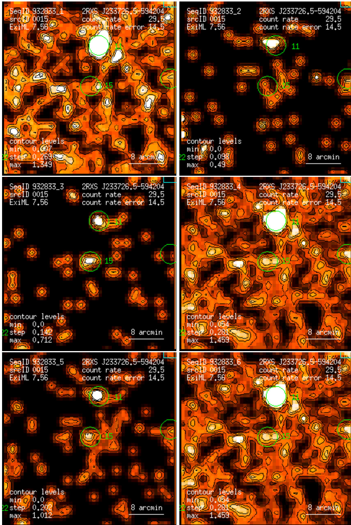
Figure 15: RASS 932833: detection 0015: band rate images, Gaussian filter: (1) PSPC channels 11 – 41, (2) 52 – 90, (3) 91 – 201, (4) 11 – 235, (5) 52 – 201, (6) 11 – 201. Broad band rates in counts/ks. Band rate contour levels in counts/ks/arcmin 2 .
