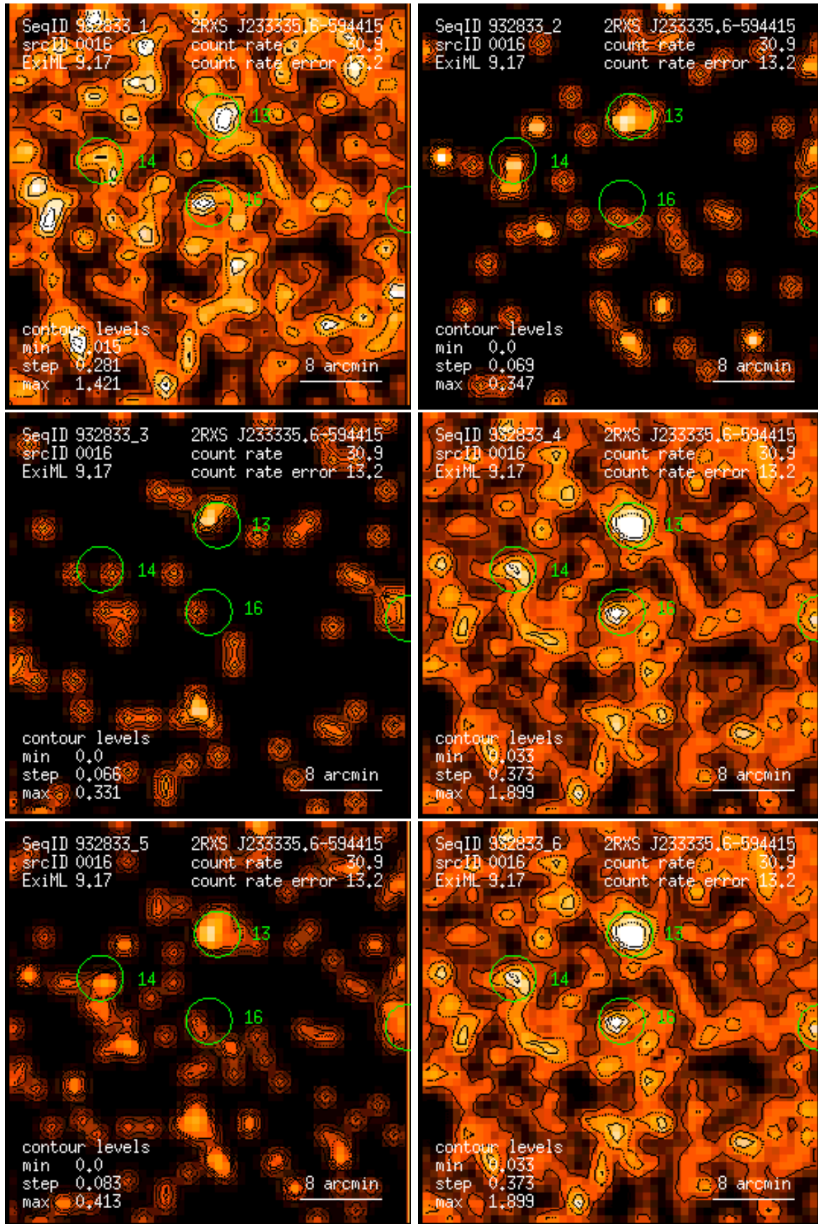
Figure 16: RASS 932833: detection 0016: band rate images, Gaussian filter: (1) PSPC channels 11 – 41, (2) 52 – 90, (3) 91 – 201, (4) 11 – 235, (5) 52 – 201, (6) 11 – 201. Broad band rates in counts/ks. Band rate contour levels in counts/ks/arcmin 2 .
