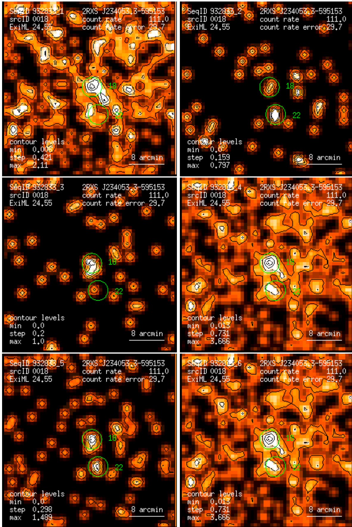
Figure 18: RASS 932833: detection 0018: band rate images, Gaussian filter: (1) PSPC channels 11 – 41, (2) 52 – 90, (3) 91 – 201, (4) 11 – 235, (5) 52 – 201, (6) 11 – 201. Broad band rates in counts/ks. Band rate contour levels in counts/ks/arcmin 2 .
