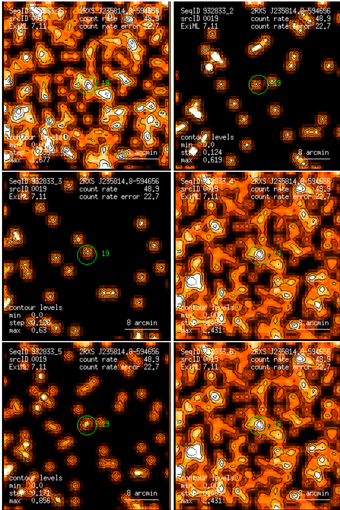
Figure 19: RASS 932833: detection 0019: band rate images, Gaussian filter: (1) PSPC channels 11 – 41, (2) 52 – 90, (3) 91 – 201, (4) 11 – 235, (5) 52 – 201, (6) 11 – 201. Broad band rates in counts/ks. Band rate contour levels in counts/ks/arcmin 2 .
