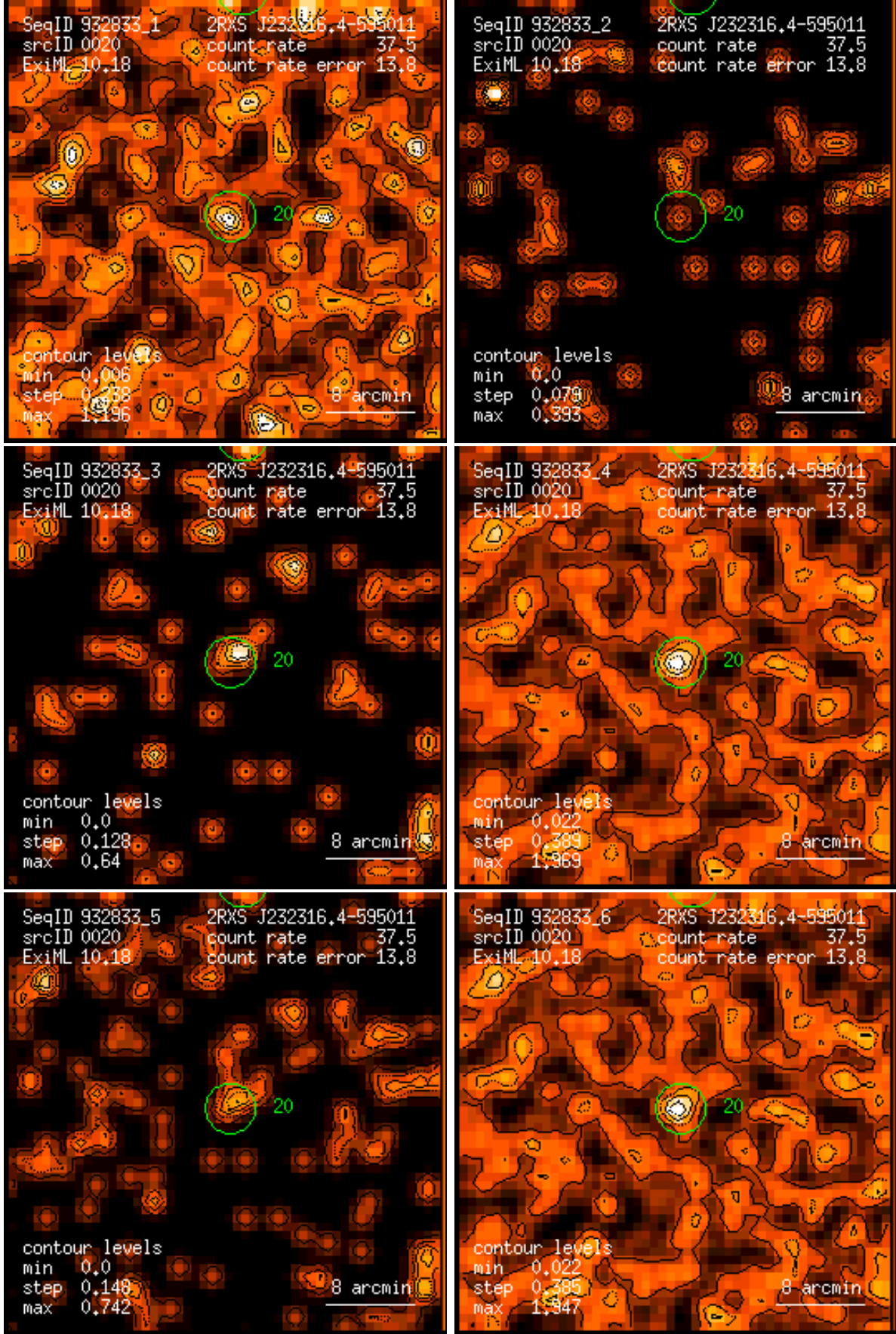
Figure 20: RASS 932833: detection 0020: band rate images, Gaussian filter: (1) PSPC channels 11 – 41, (2) 52 – 90, (3) 91 – 201, (4) 11 – 235, (5) 52 – 201, (6) 11 – 201. Broad band rates in counts/ks. Band rate contour levels in counts/ks/arcmin 2 .
