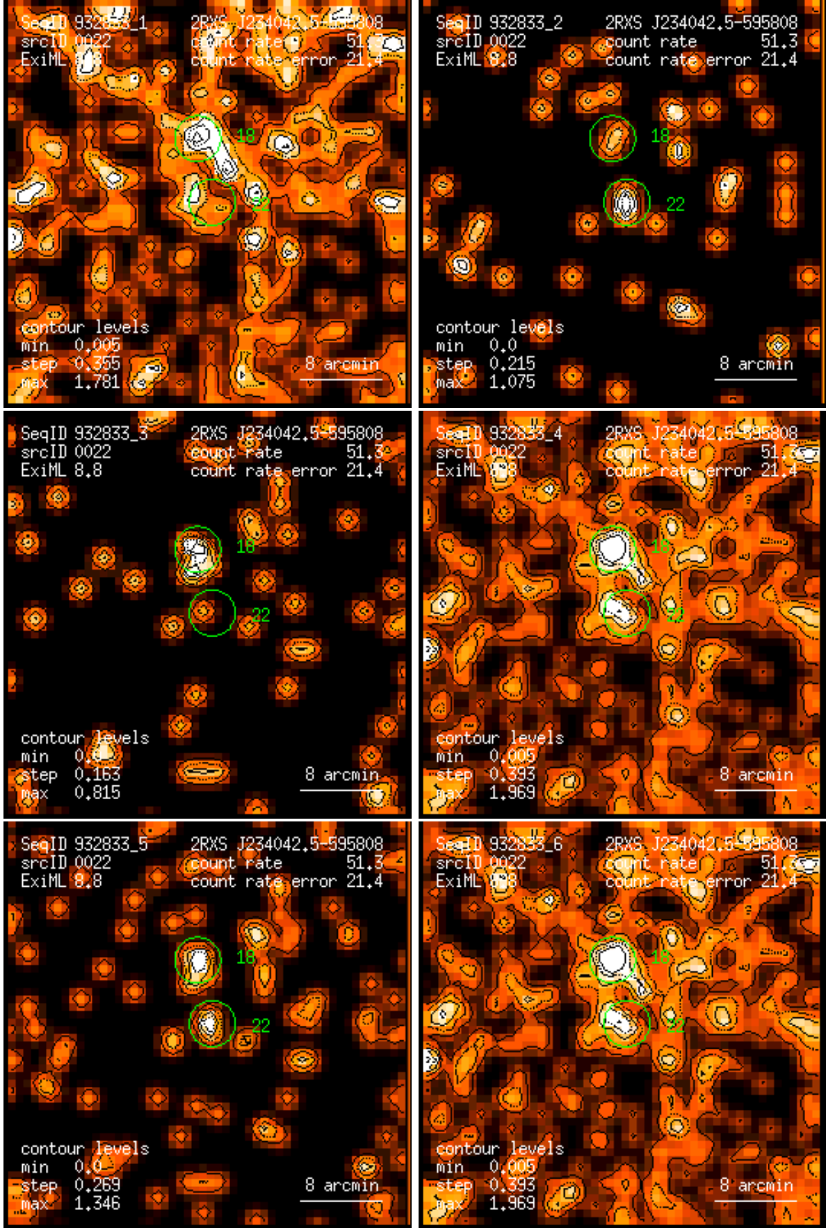
Figure 22: RASS 932833: detection 0022: band rate images, Gaussian filter: (1) PSPC channels 11 – 41, (2) 52 – 90, (3) 91 – 201, (4) 11 – 235, (5) 52 – 201, (6) 11 – 201. Broad band rates in counts/ks. Band rate contour levels in counts/ks/arcmin 2 .
