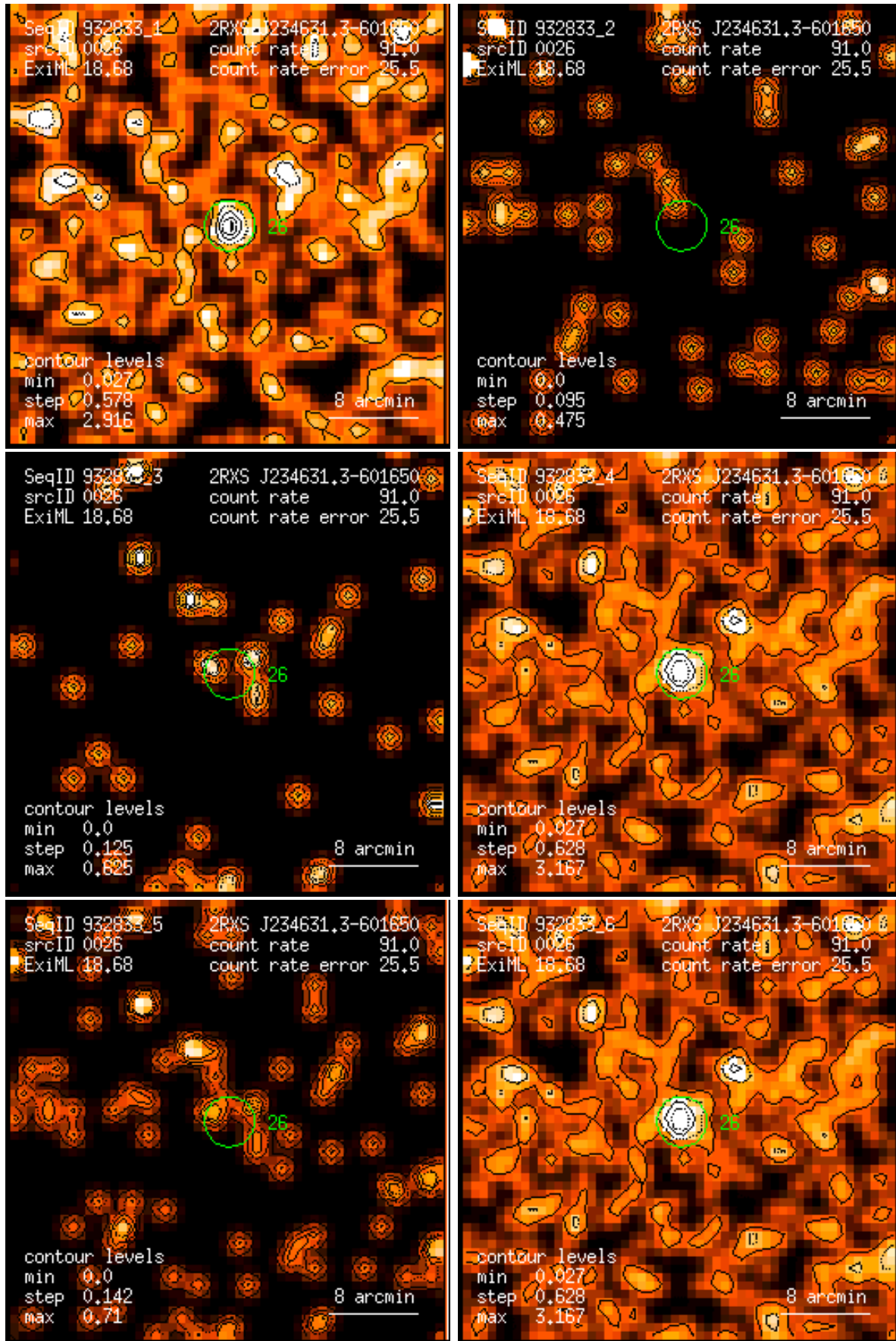
Figure 26: RASS 932833: detection 0026: band rate images, Gaussian filter: (1) PSPC channels 11 – 41, (2) 52 – 90, (3) 91 – 201, (4) 11 – 235, (5) 52 – 201, (6) 11 – 201. Broad band rates in counts/ks. Band rate contour levels in counts/ks/arcmin 2 .
